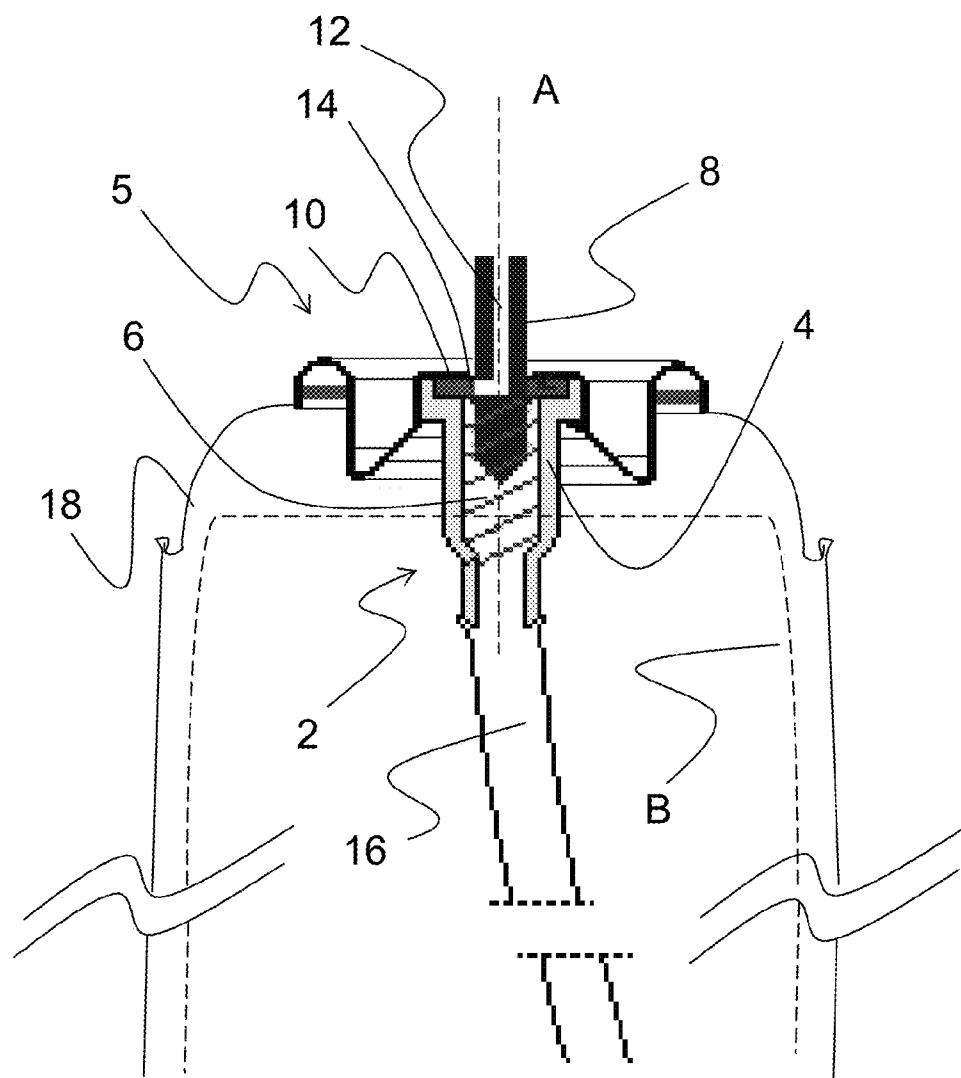
FIG. 3 (PRIOR ART)
