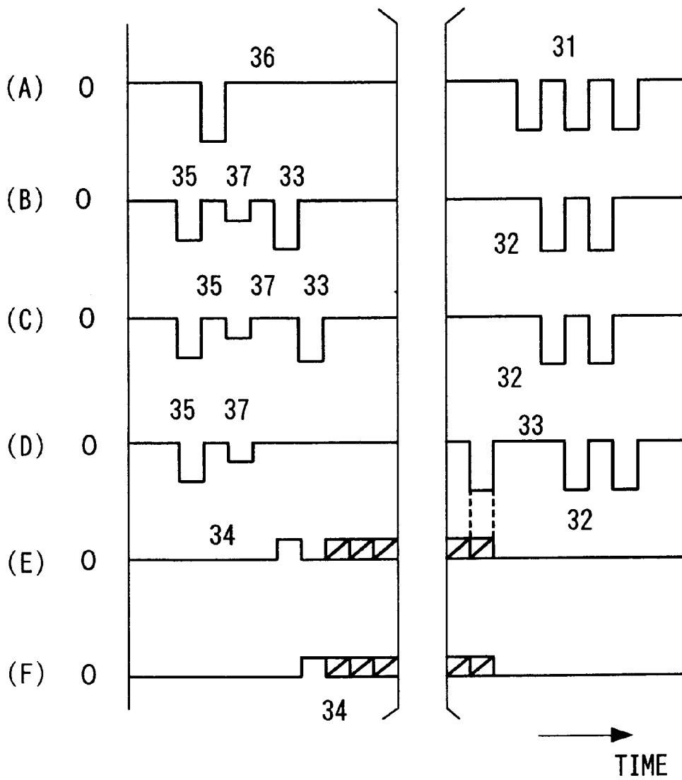
SUB-FIELD PANEL DRIVE VOLTAGE OF FIFTH EMBODIMENT
