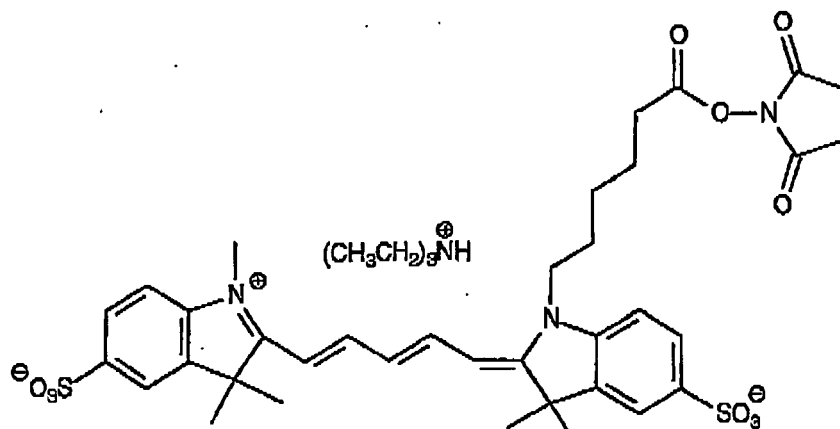
Compound 30
