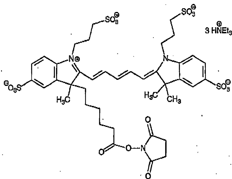
Compound 9
