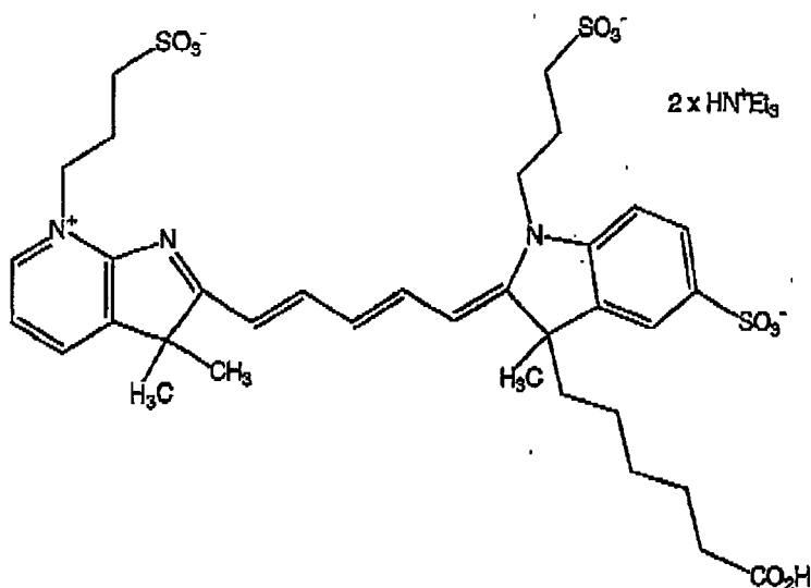
Compound 68
