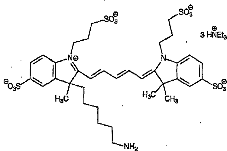
Compound 17
