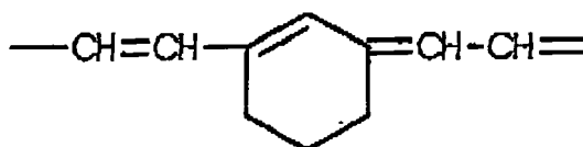
Formula IX
