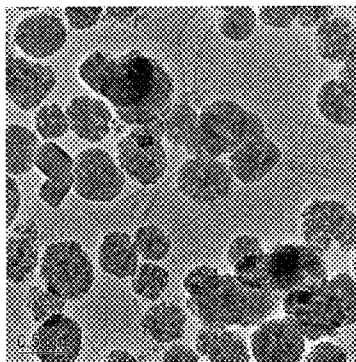
TEM of carbon nanosphere templated mesoporous silica-1 after calcination.
