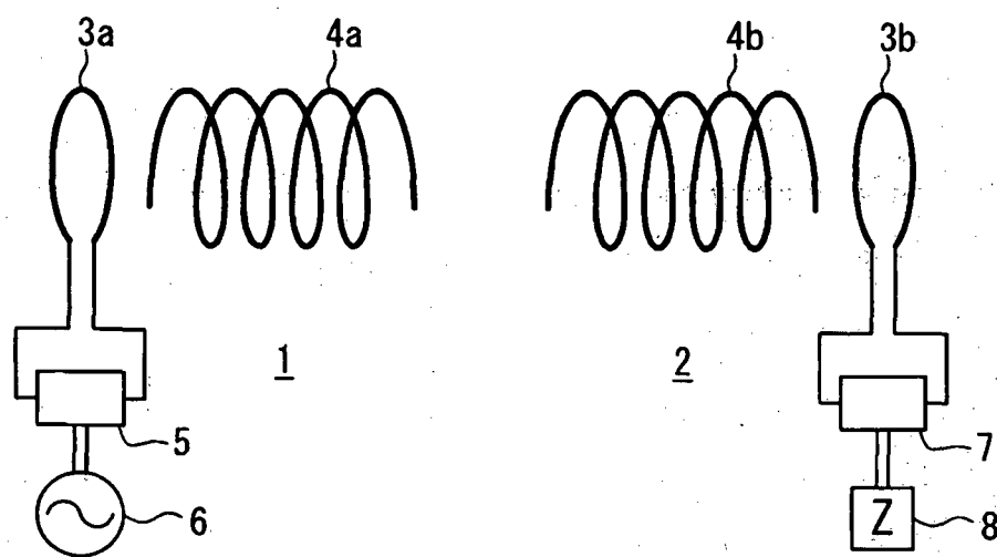
FIG. 17 PRIOR ART
