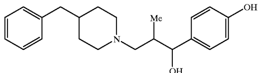
\alpha -(4-hydroxyphenyl)- \beta -methyl(phenylmethyl)-1-piperidinepropanol.
