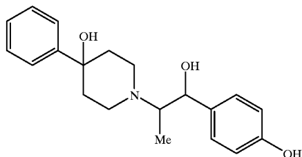
4-hydroxy- \alpha -(4-hydroxyphenyl)- \beta -methyl-4-phenyl-1-piperidineethanol;
