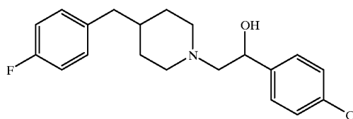
\alpha -(4-chlorophenyl)-4-[(4-fluorophenyl)methyl]-1-piperidineethanol (Eliprodil, available from Synthelabo, Inc., and disclosed in U.S. Pat. No. 5,547,963)
