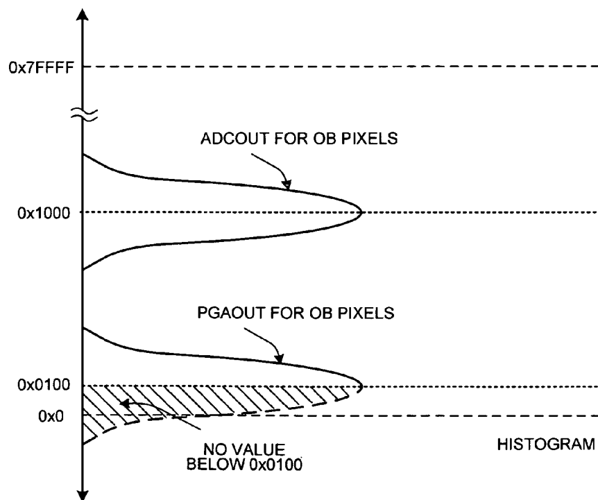
OB PIXEL NOISE DISTRIBUTION CURVE
