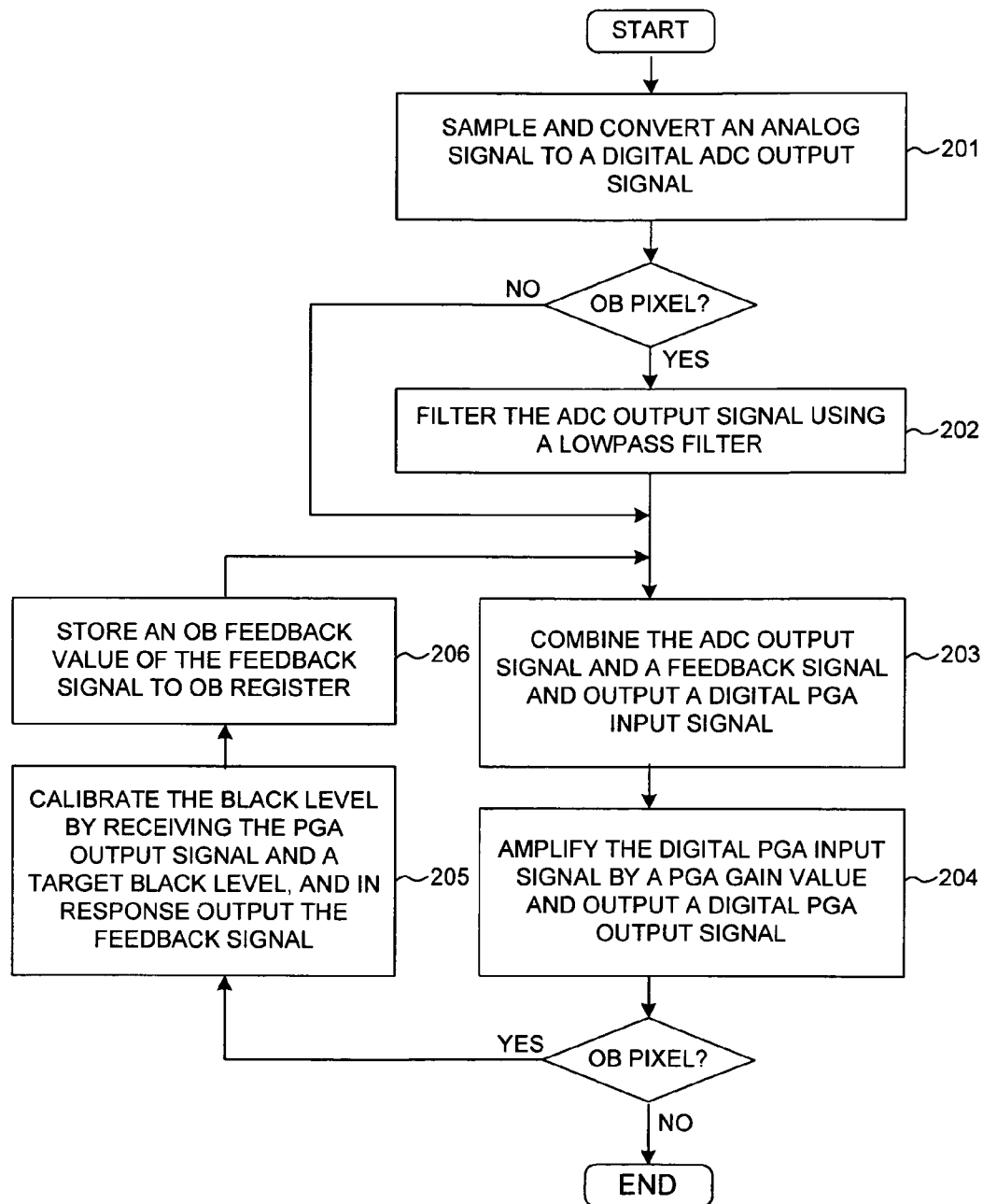
BLACK LEVEL CALIBRATION WITH FEEDBACK CONTROL
