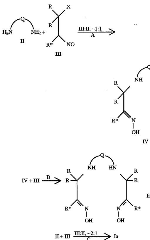
Reaction Scheme 1 Preparation of Compounds of the Formula Ia
