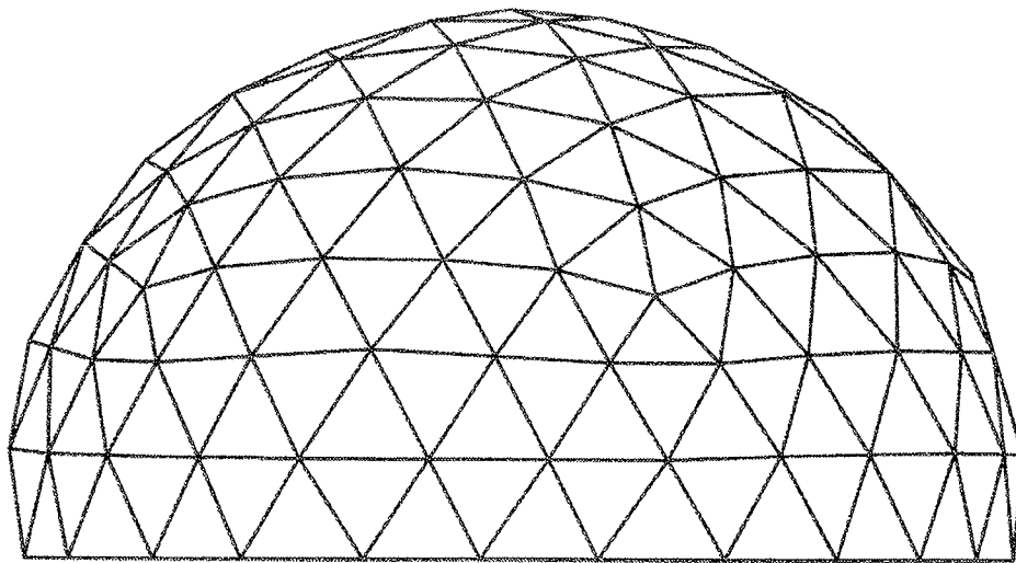
Geodesic 5V 8/15 Icosahedron Dome Pattern
