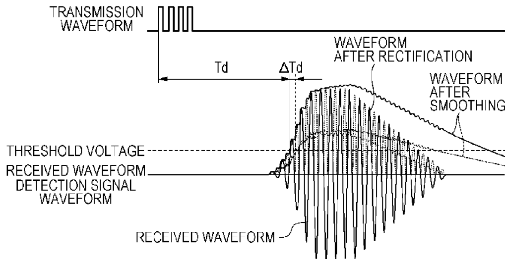
FULL WAVE RECTIFYING DETECTION
