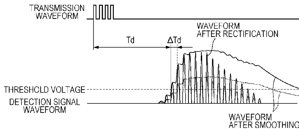
HALF WAVE RECTIFYING DETECTION
