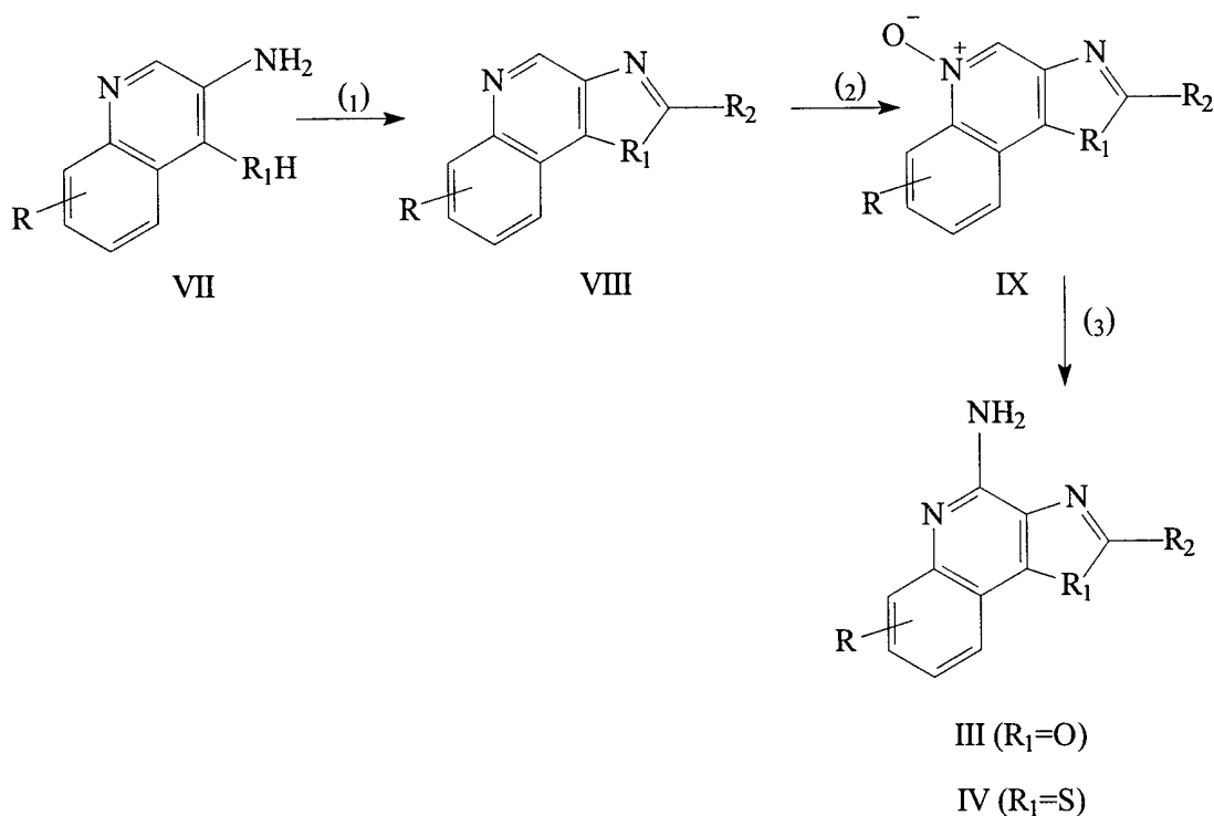
Reaction Scheme II
