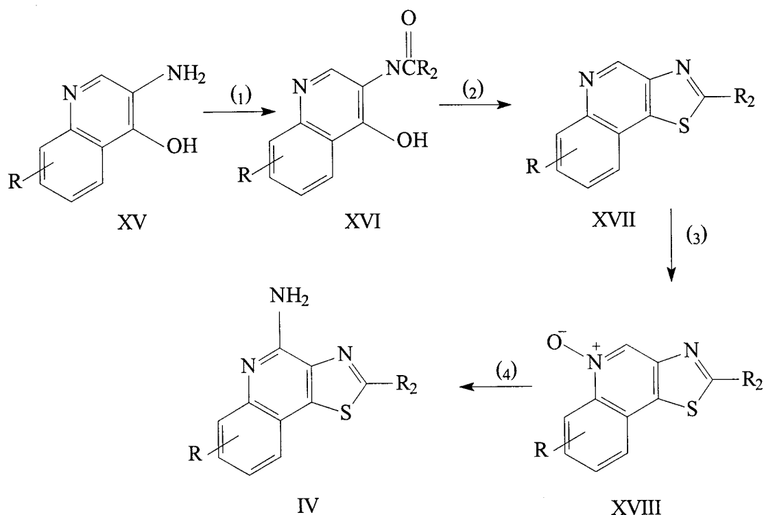
Reaction Scheme IV
