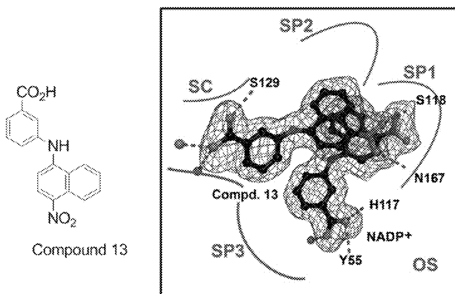
Double-decker AKR1C3 structure
