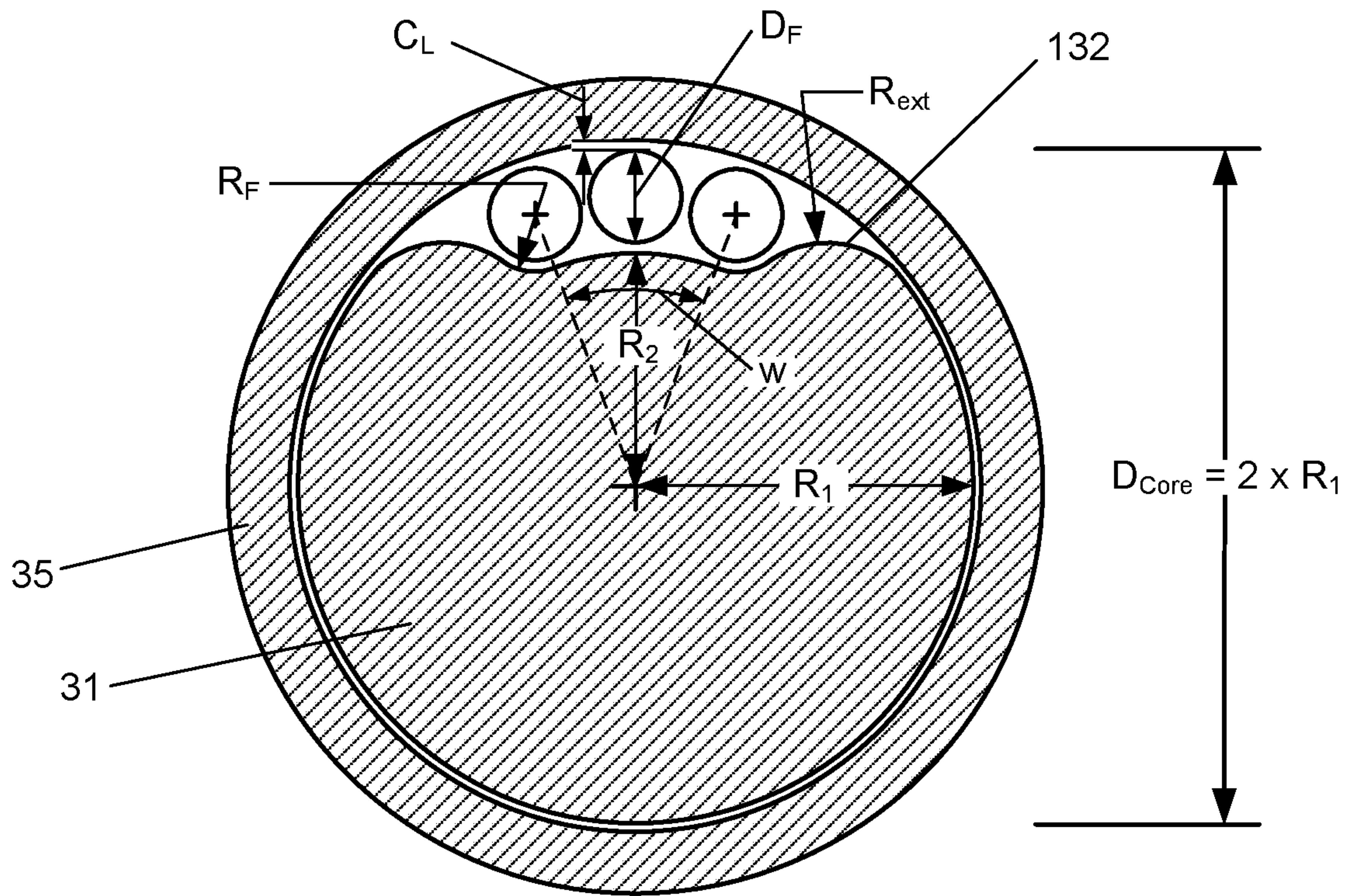
B-B CUT-THROUGH VIEW OF FIG. 5A
