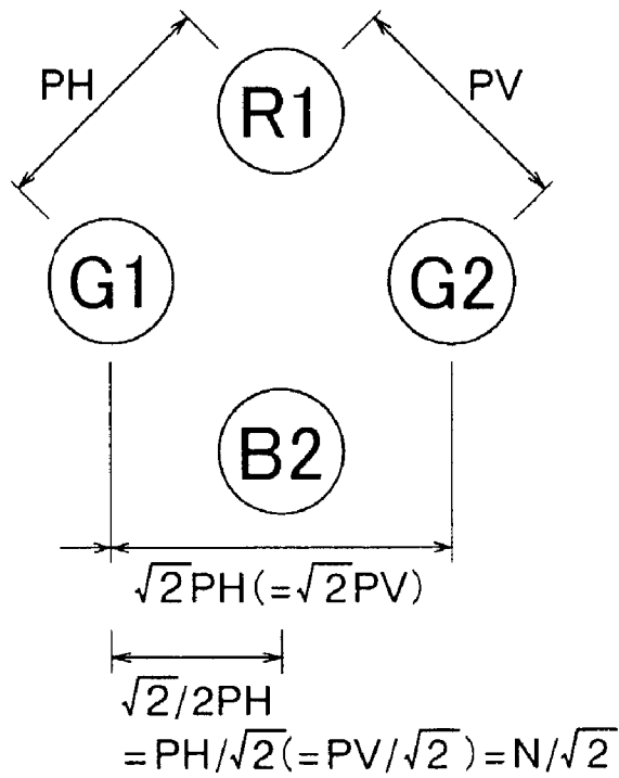
FIG. 13 PRIOR ART
