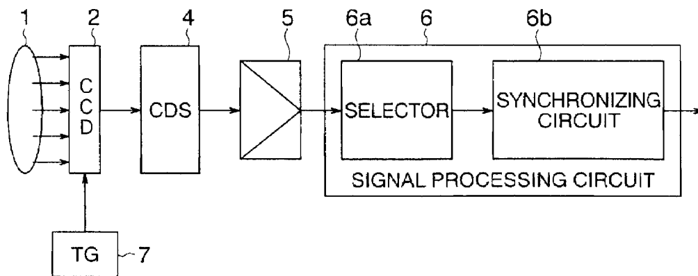
FIG. 4 PRIOR ART
