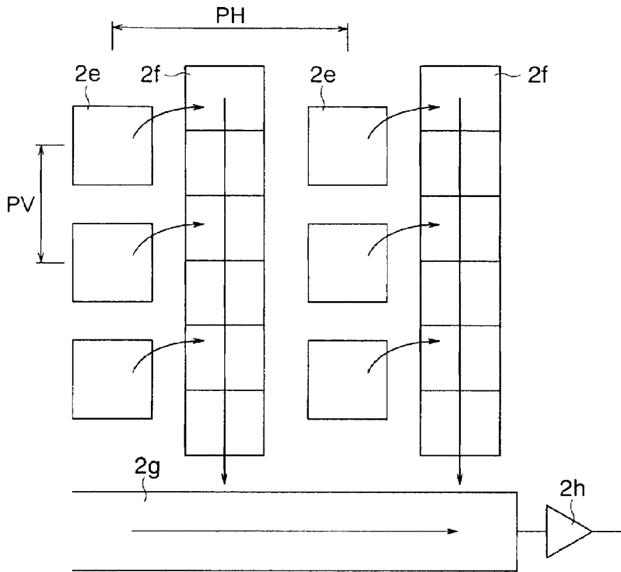
FIG. 3 PRIOR ART
