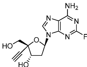
(2 R ,3 S ,5 R )-5-(6-amino-2-fluoro-9 H -purin-9-yl)-2-ethynyl-2-(hydroxymethyl)tetrahydrofuran-3-ol
