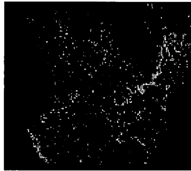
p(\text{sky} | Y)
