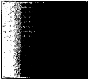
p(\text{sky} | \text{pos})
