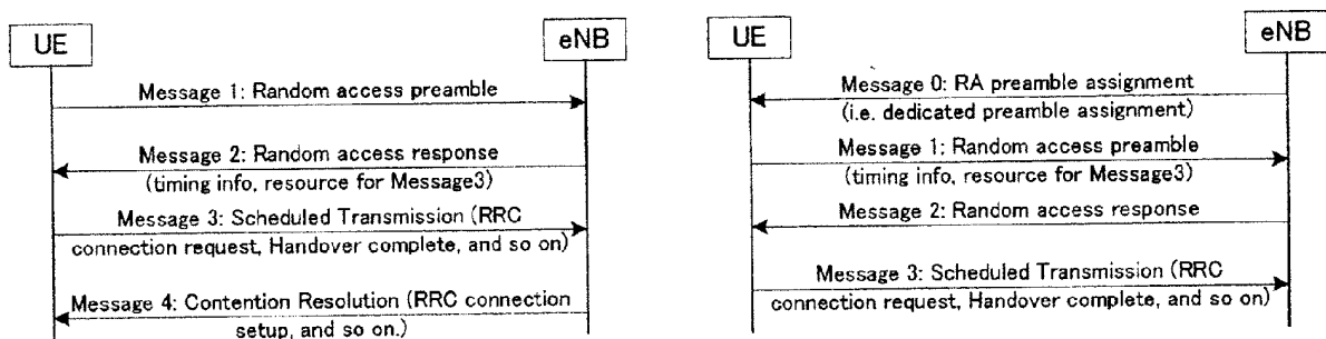
(b) dedicated RACH preamble case
