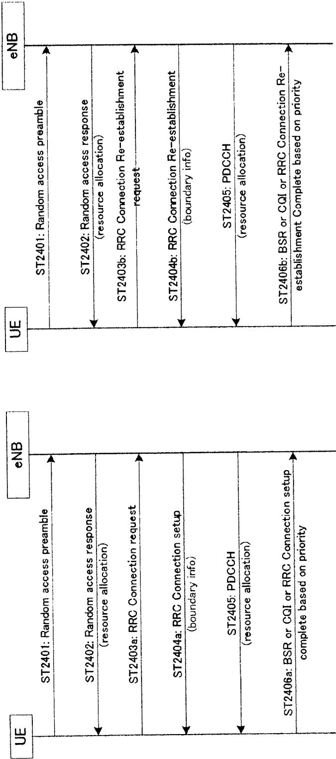
(a) RRC connection establishment procedure
