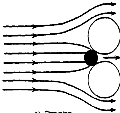
a) Straining
