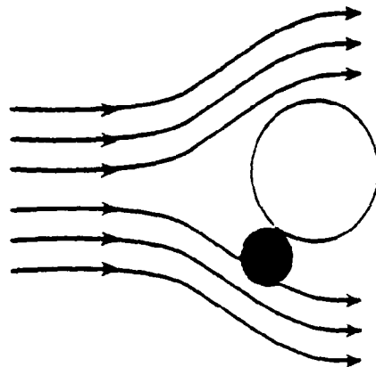
c) Interaction
