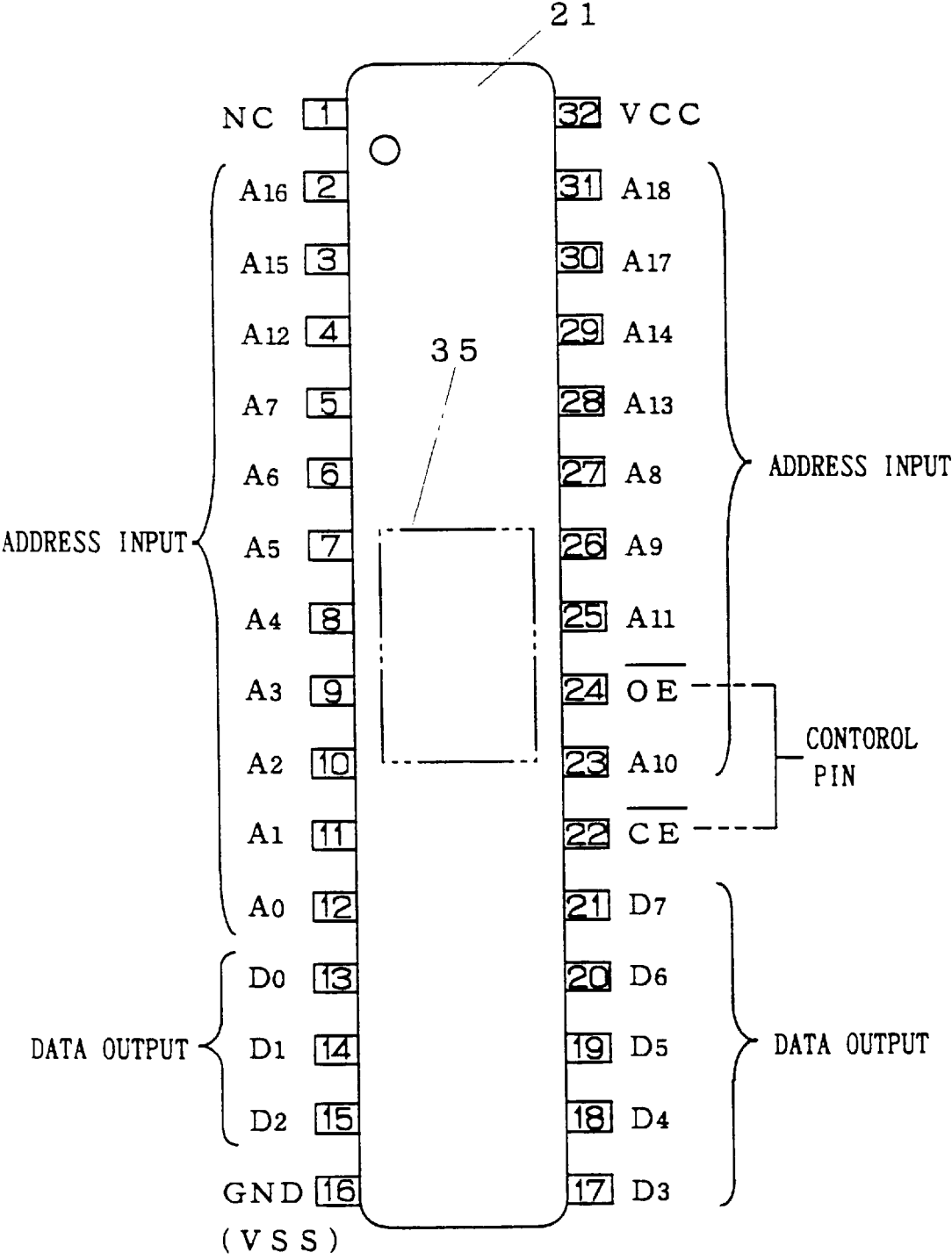
FIG. 10 PRIOR ART
