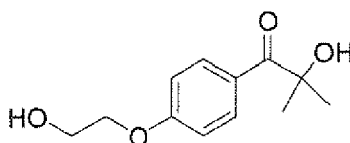
IRGACURE 2959
