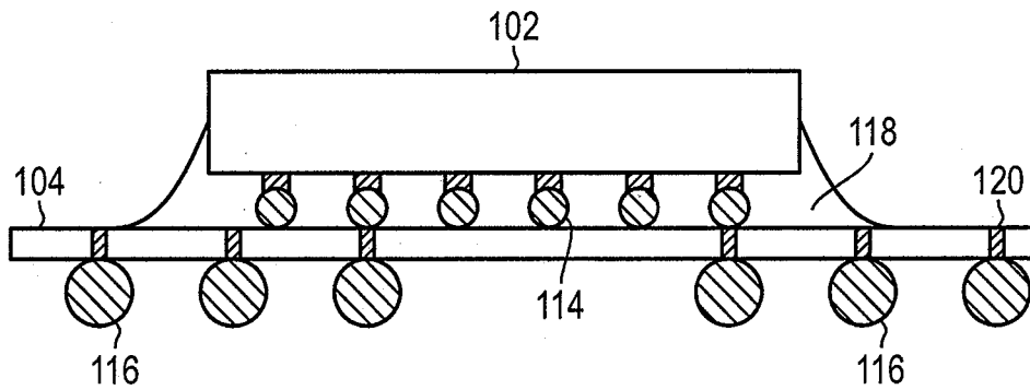
FIG. 2 (PRIOR ART)
