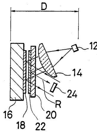
FIG. 15 PRIOR ART
