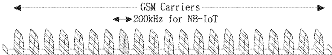
Standalone Mode
