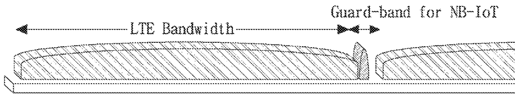
Guard-band Mode
