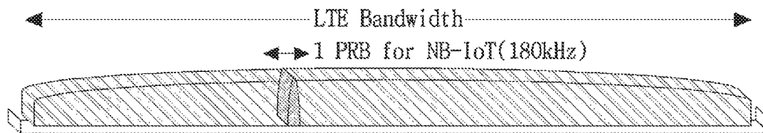
In-band Mode
