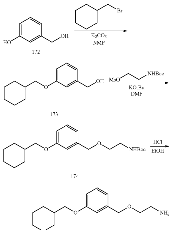
SCHEME 53
