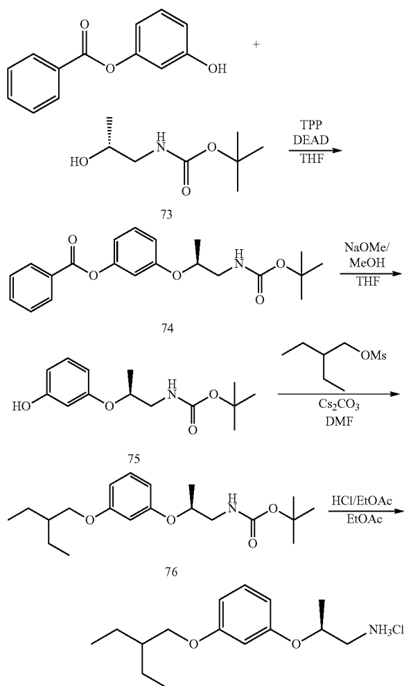
SCHEME 21
