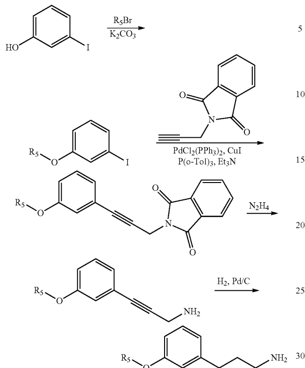
SCHEME I
