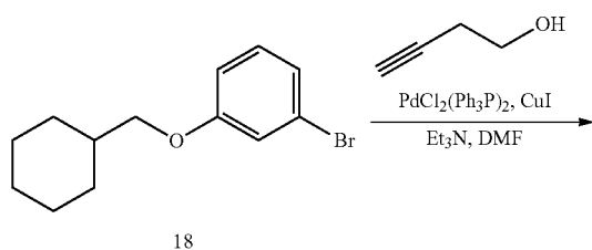
SCHEME 52
