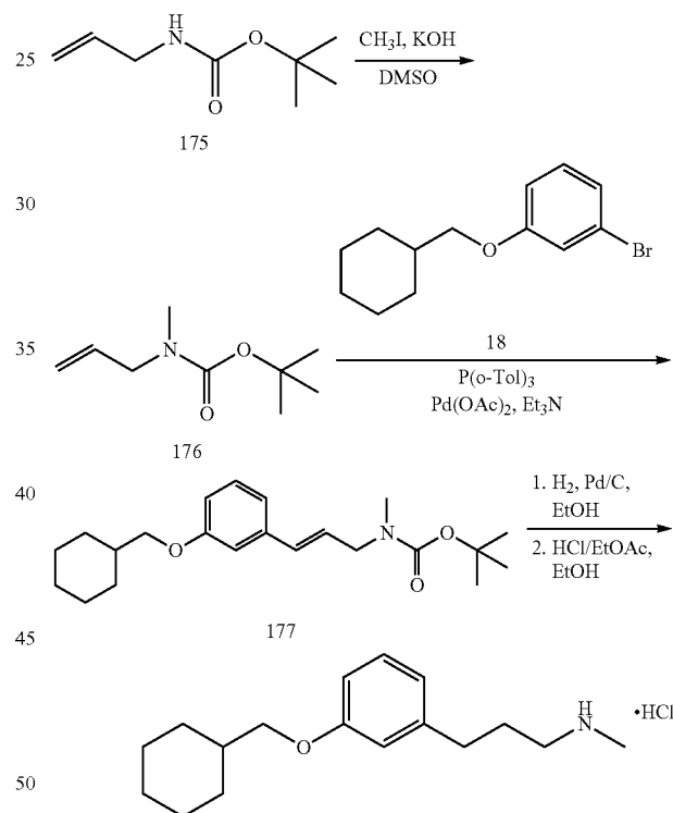
SCHEME 54
