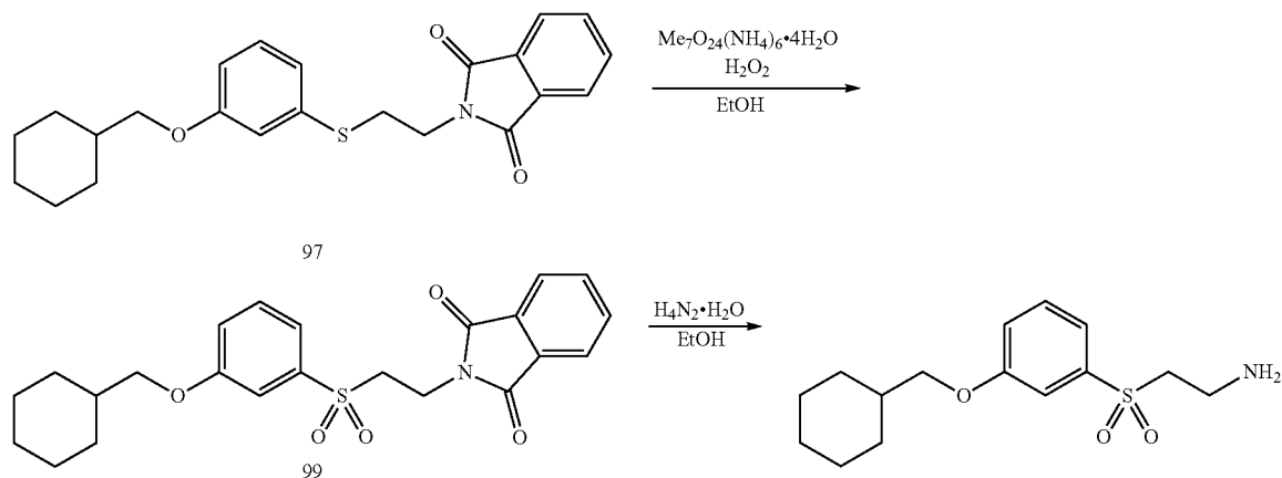
SCHEME 33
