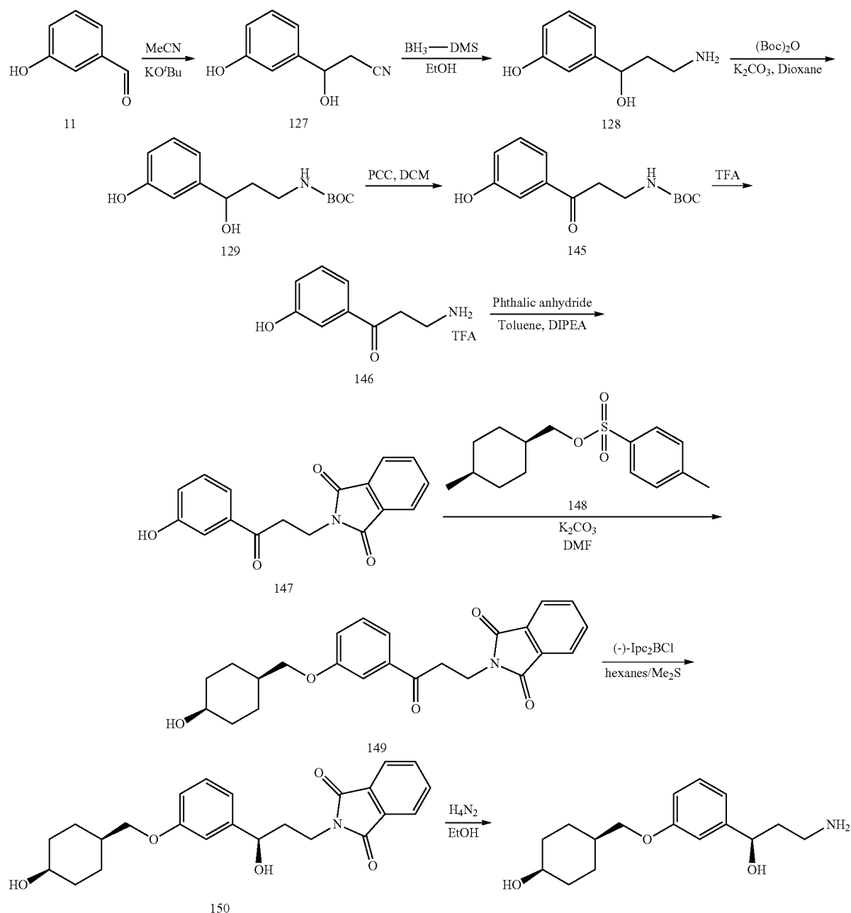
SCHEME 47
