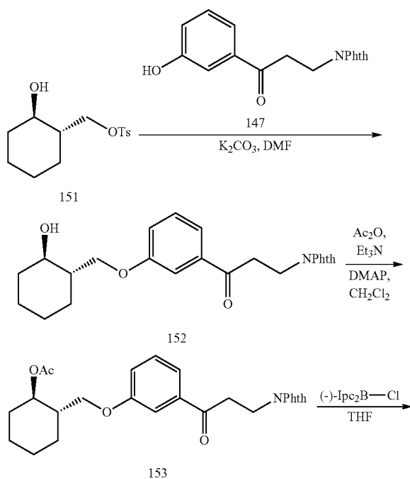
SCHEME 48
