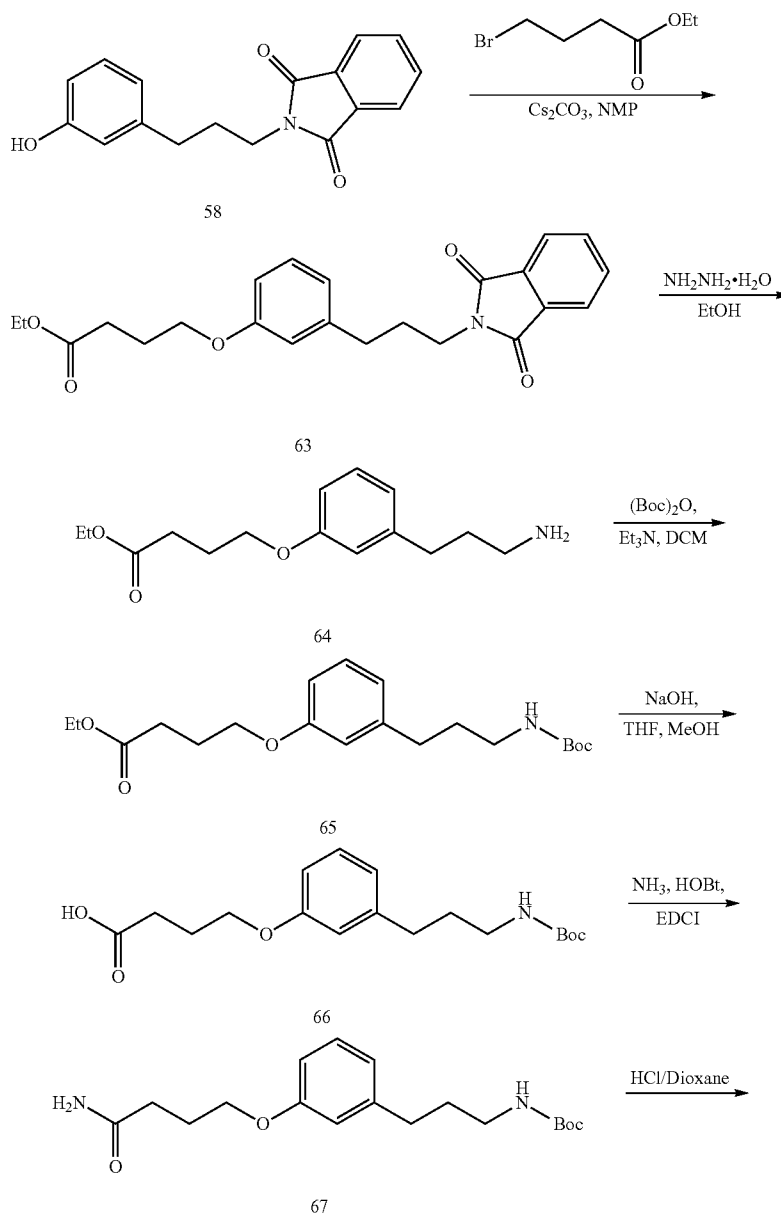
SCHEME 19
