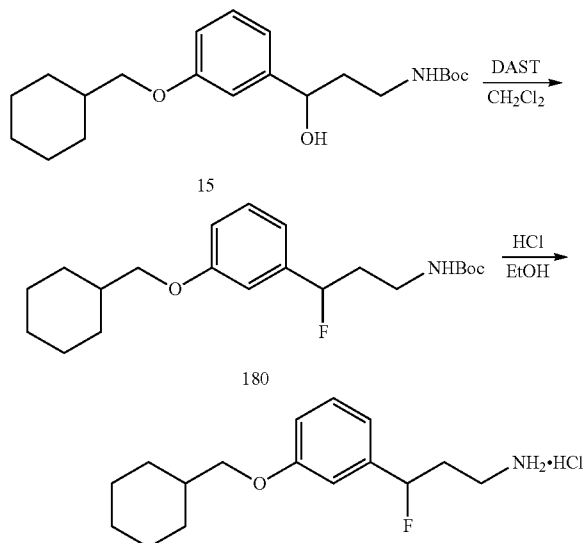
SCHEME 58
