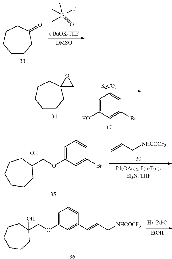
SCHEME 8
