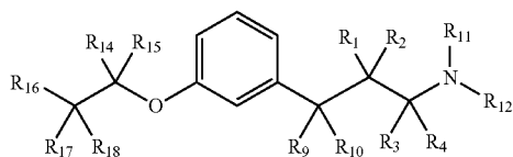
Formula (IIa)
