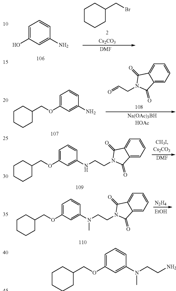
SCHEME 36
