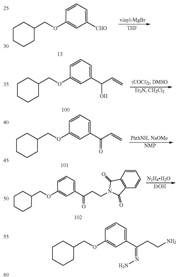
SCHEME 34
