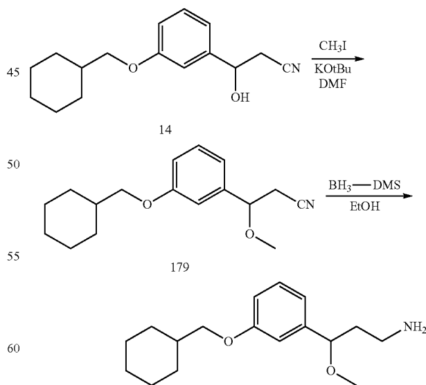
SCHEME 57
