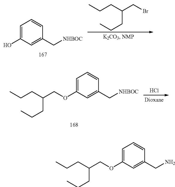
SCHEME 51
