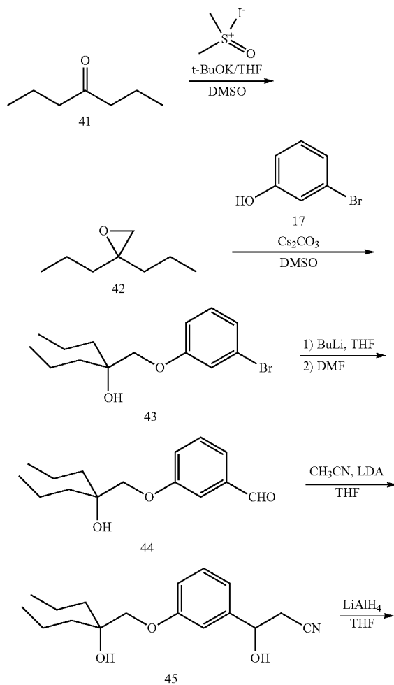
SCHEME 12
