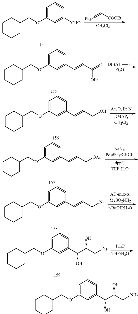
SCHEME 49
