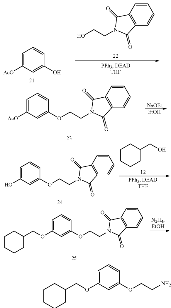
SCHEME 6
