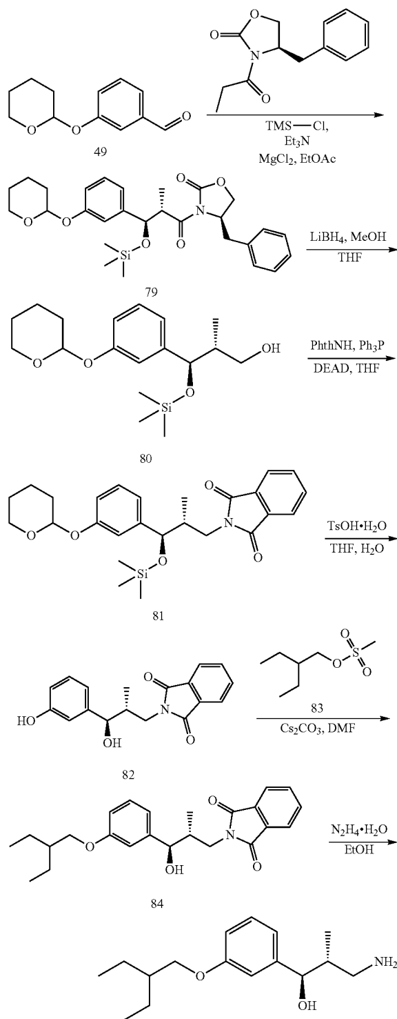
SCHEME 23
