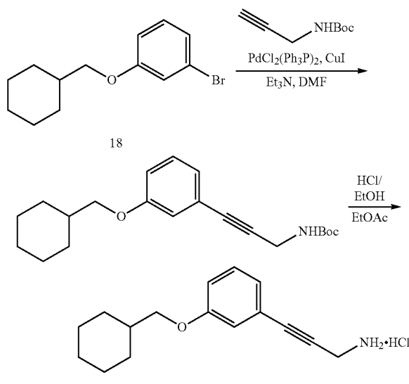
SCHEME 57
