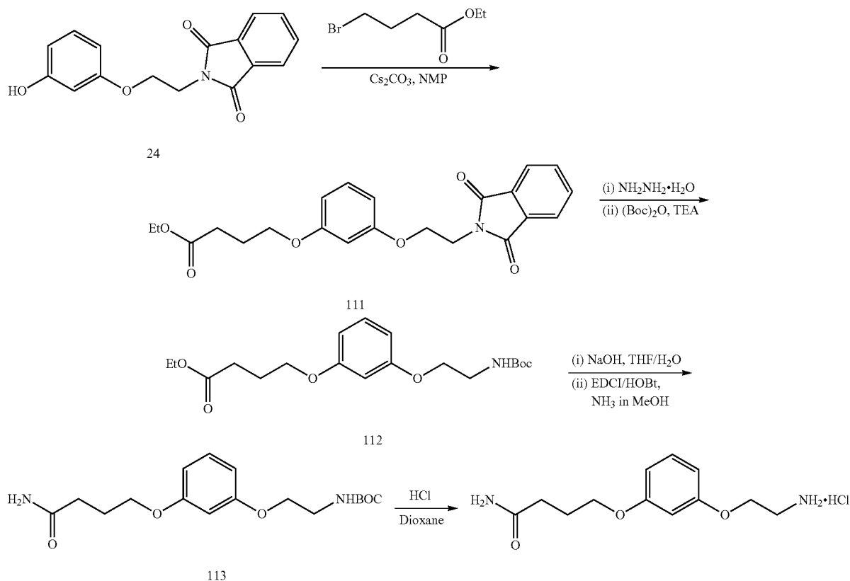
SCHEME 38
