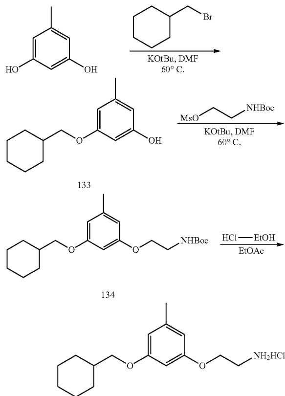
SCHEME 43
