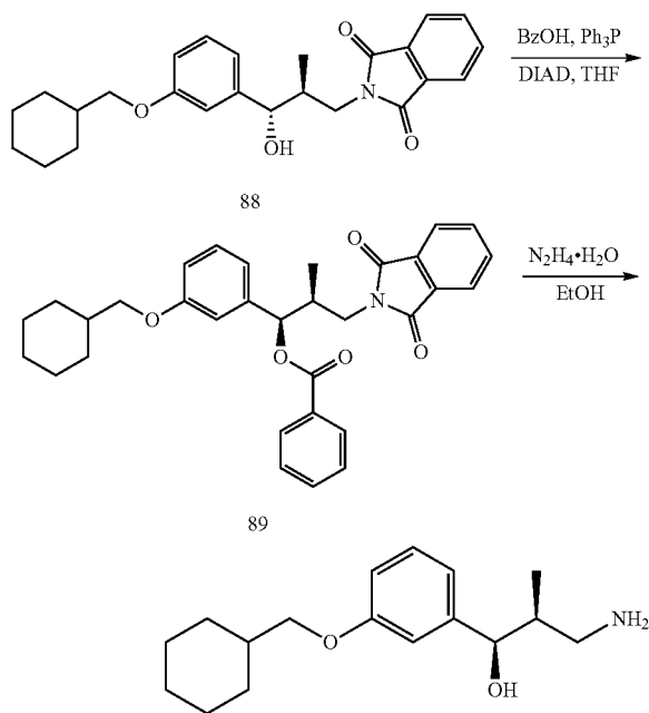
SCHEME 25
