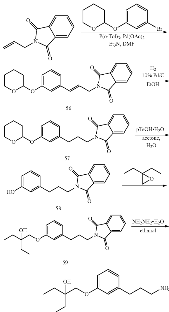
SCHEME 16
