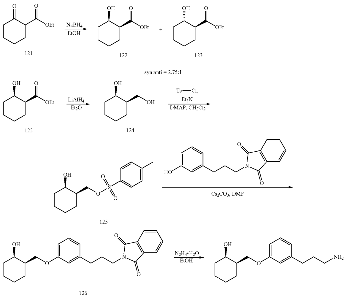
SCHEME 41
