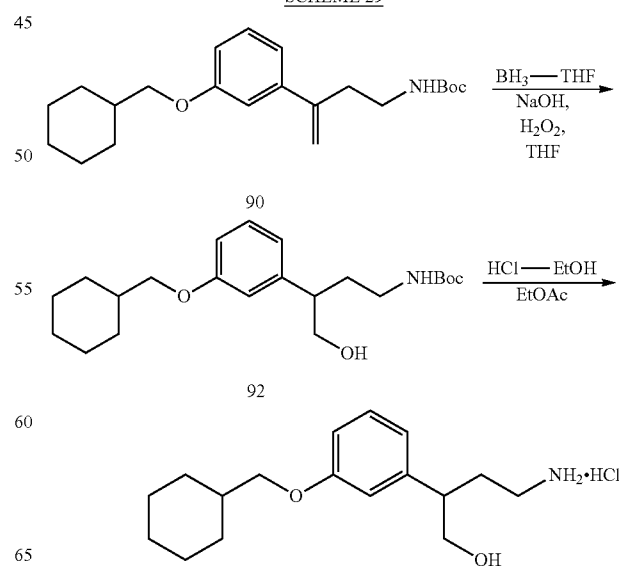
SCHEME 29
