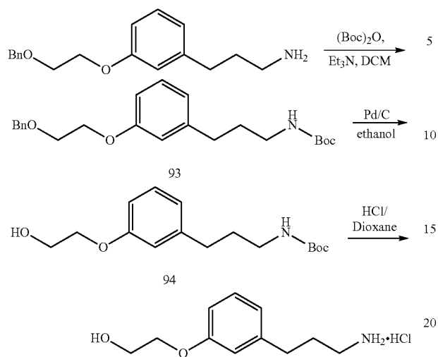
SCHEME 30
