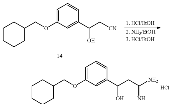
SCHEME 37
