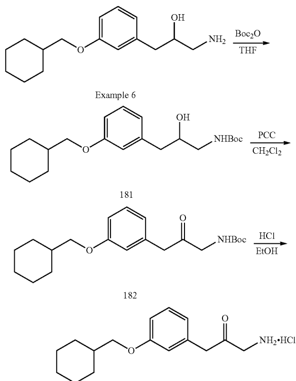
SCHEME 59
