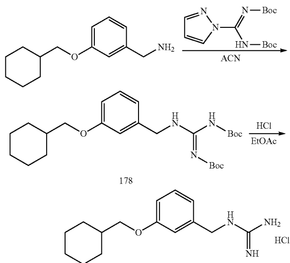
SCHEME 56
