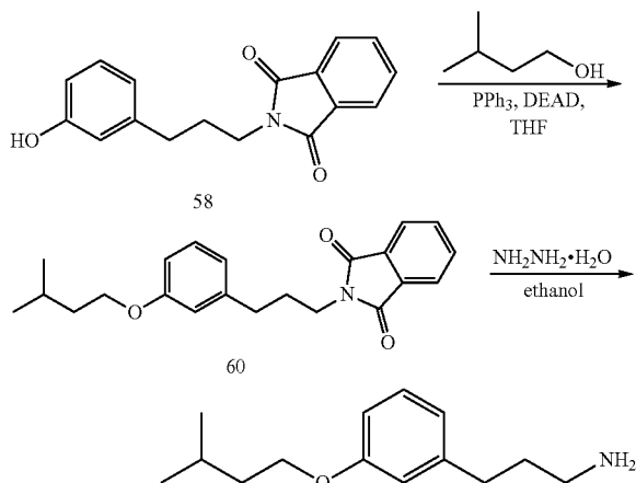
SCHEME 17
