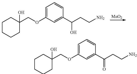
SCHEME 13
