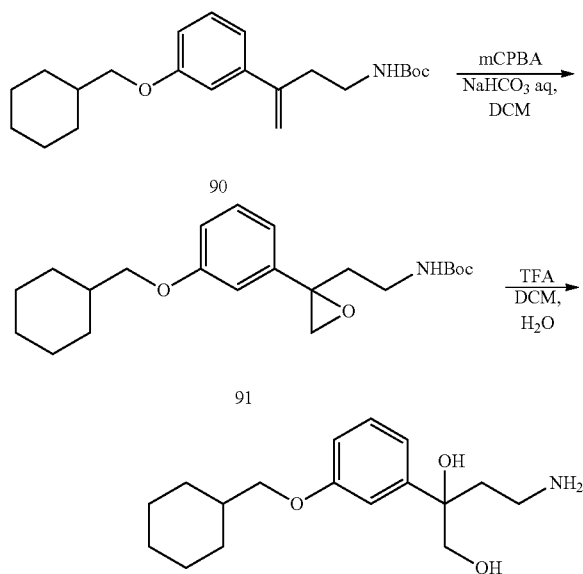
SCHEME 28
