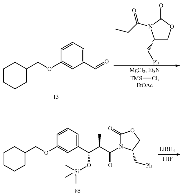
SCHEME 24
