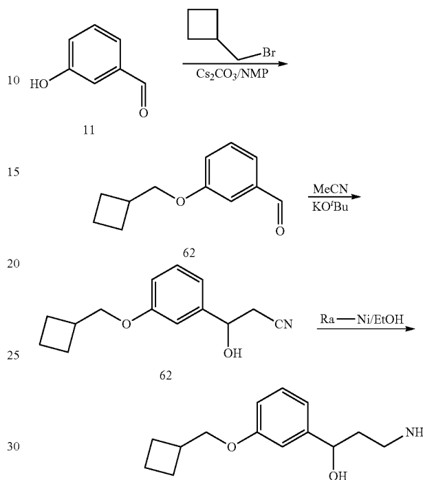
SCHEME 18
