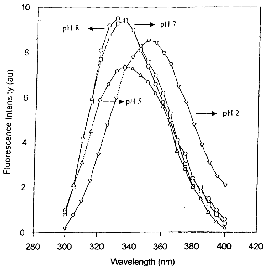
Fluorescence Spectrum Of Thrombinase
