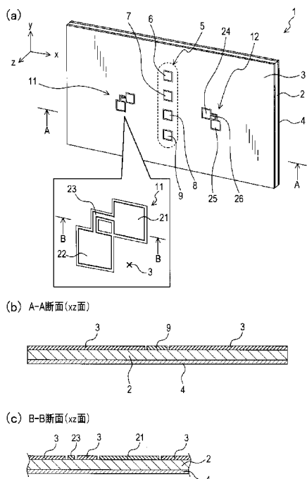
(b) A-A cross-section (xz plane) (c) B-B cross-section (xz plane)
