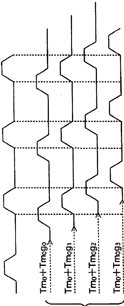
FIG. 7C OUTPUT FROM SECOND DELAY PROCESSING SUB-UNIT
