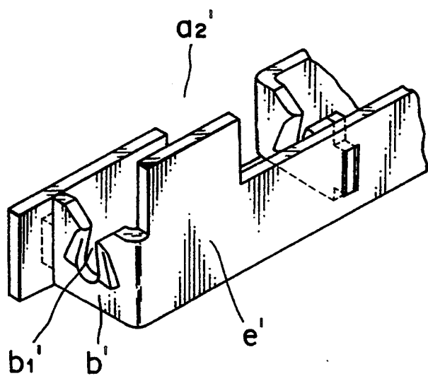
FIG. 6 PRIOR ART
