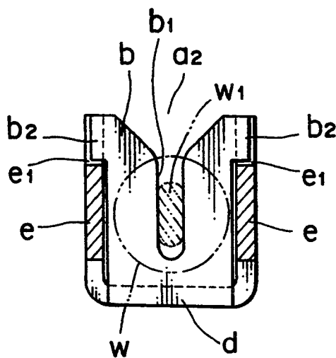
FIG. 5 PRIOR ART
