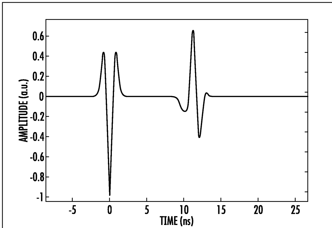
FIG. 3C PRIOR ART
