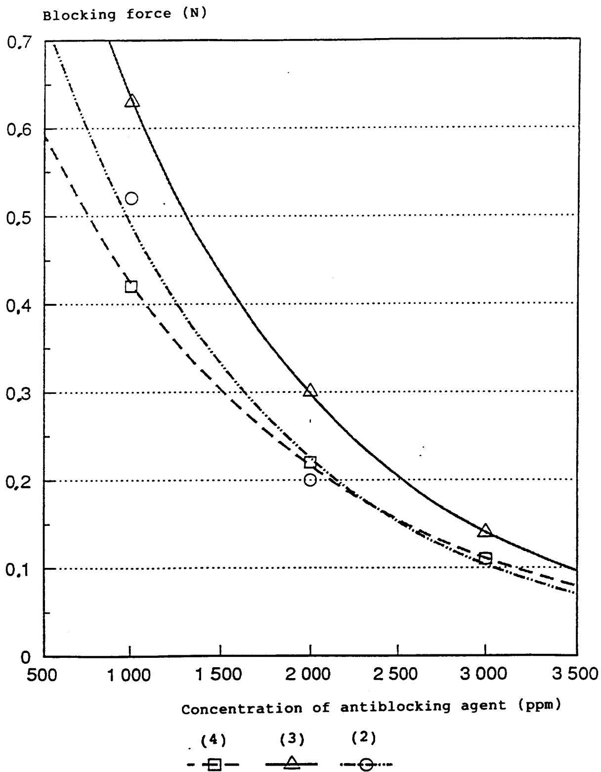
Figure 3 Antiblocking behaviour
