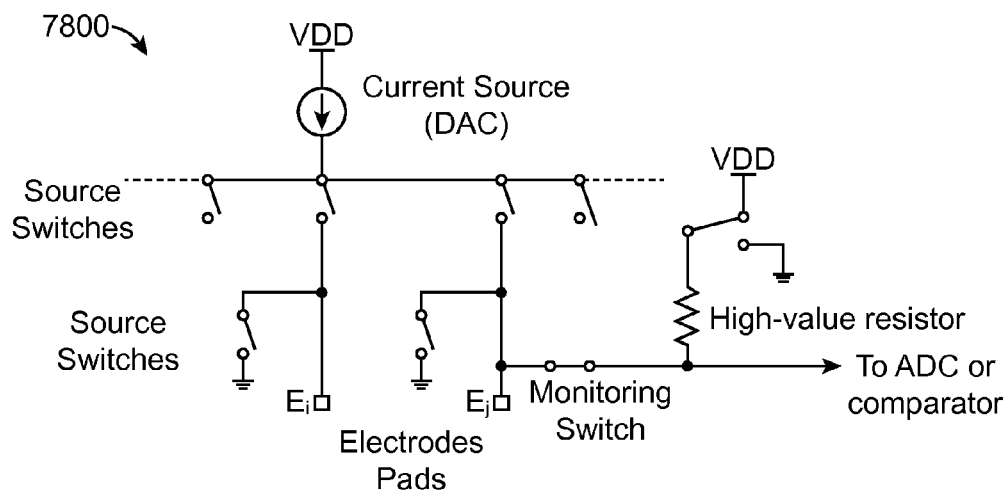
Leakage Monitoring Scheme
