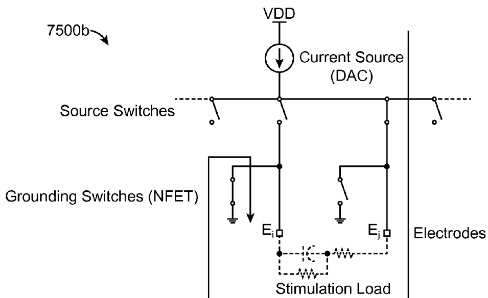
Single-channel Stimulator, Recovery Phase
