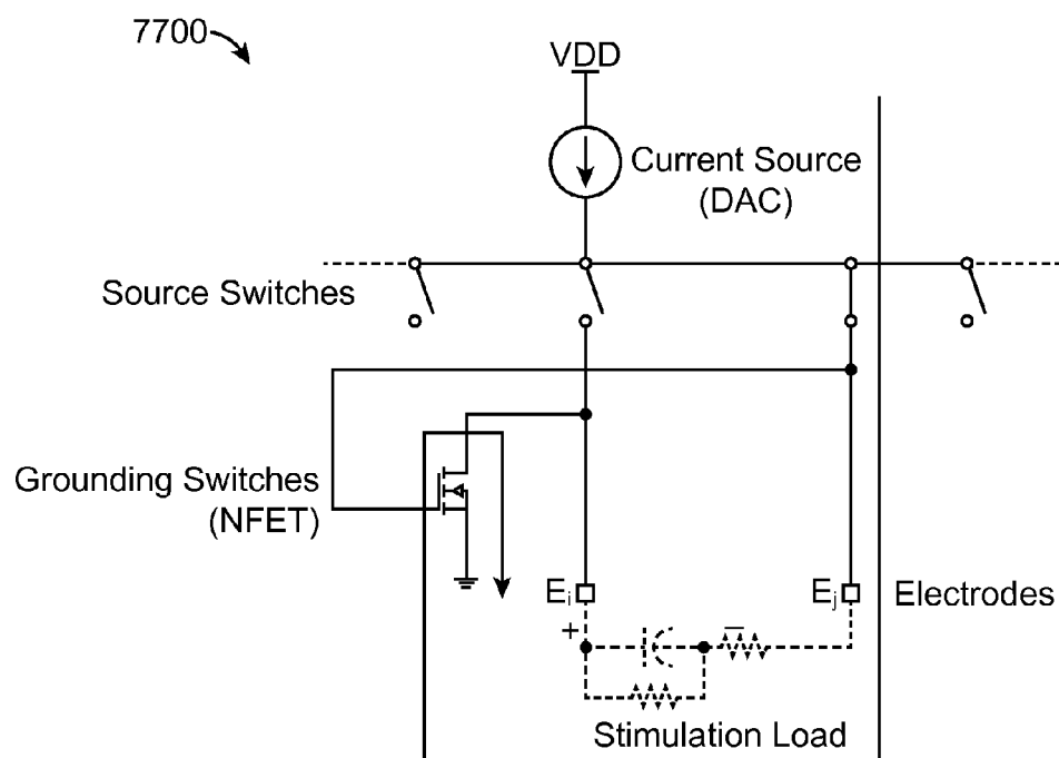
Grounding Load, Recovery Phase
