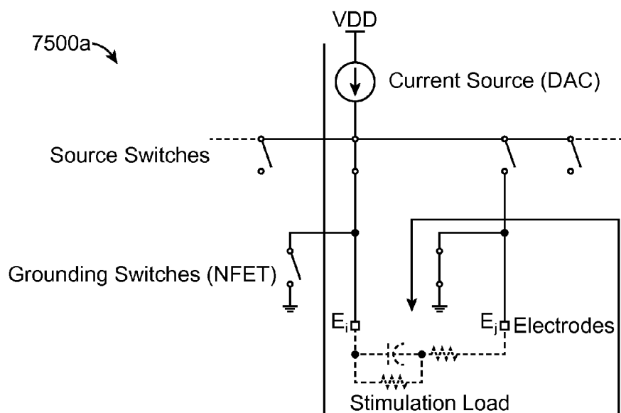
Single-channel Stimulator, Stimulation Phase
