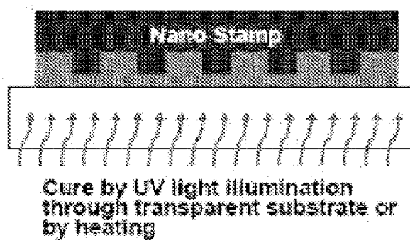
(b) UV-cure of PDMS
