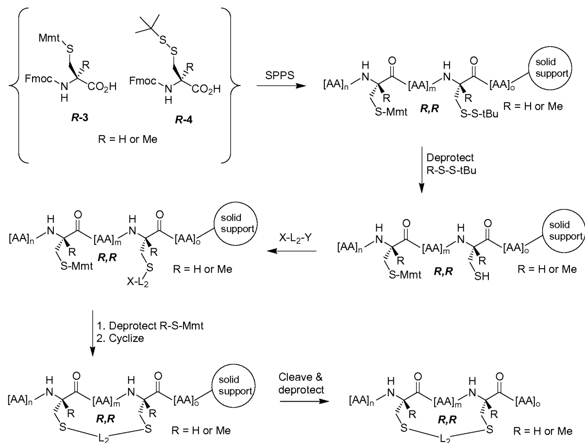
Synthetic Scheme 8:
