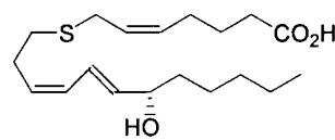
5 (15S)-(5Z,11Z,13E)-15-hydroxy-8-thia-5,11,13-eicosatrienoic acid
