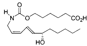
8 (15S)-(11Z,13E)-9-aza-15-hydroxy-7-oxa-8-oxo-11,13-eicosadienoic acid
