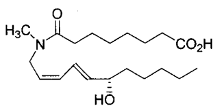
6 (15S)-(11Z,13E)-9-aza-15-hydroxy-9-methyl-8-oxo-11,13-eicosadienoic acid
