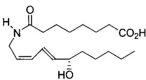
7 (15S)-(11Z,13E)-9-aza-15-hydroxy-8-oxo-11,13-eicosadienoic acid
