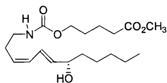
4 (15S)-(11Z,13E)-8-aza-15-hydroxy-6-oxa-7-oxo-11,13-eicosadienoic acid methyl ester
