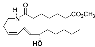
3 (15S)-(11Z,13E)-8-aza-15-hydroxy-7-oxo-11,13-eicosadienoic acid methyl ester
