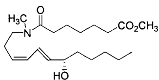
2 (15S)-(11Z,13E)-8-aza-15-hydroxy-8-methyl-7-oxo-11,13-eicosadienoic acid methyl ester
