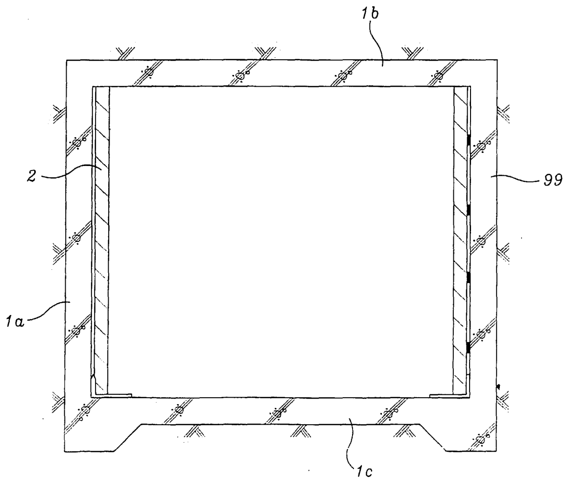
Fig. 2 conventional art.
