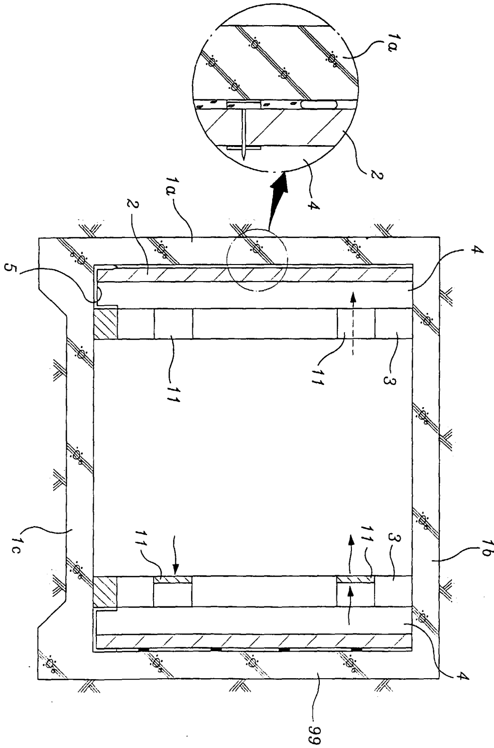
Fig. 3 conventional art
