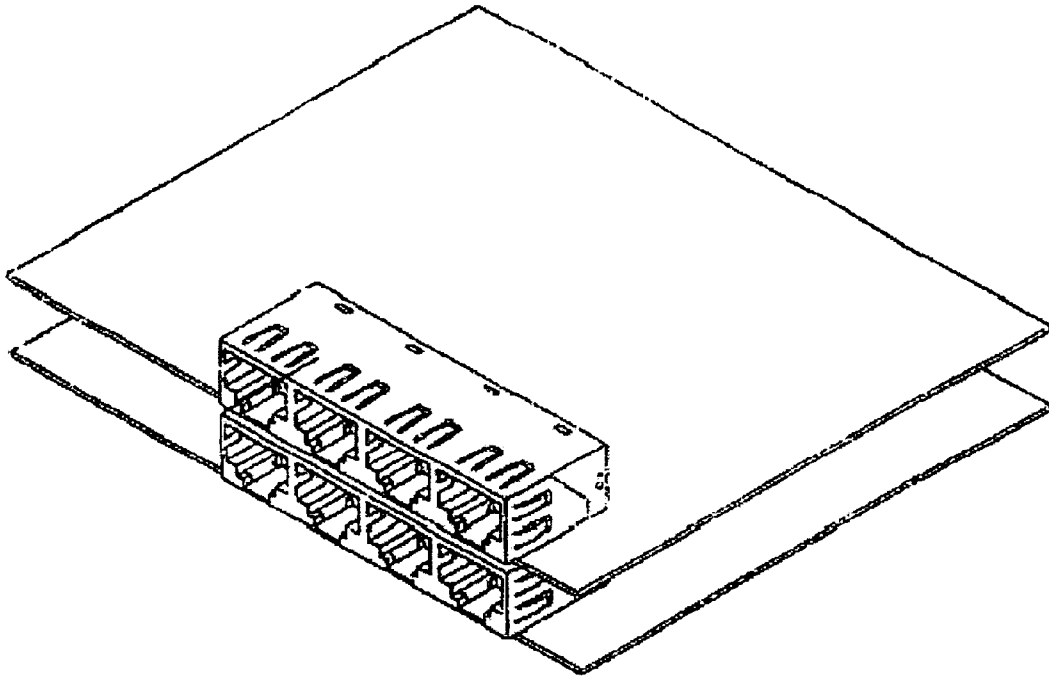
Fig. 1(a)(Prior Art)
