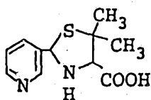
5,5-Dimethyl-2-(3-pyridyl)- thiazolidine-4-carboxylic acid
