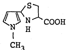
2-[3-(1-Methylpyrrolyl)]- thiazolidine-4-carboxylic acid
