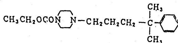
Ethyl 1-(4-methyl-4-phenylpentyl)- piperazine-4-carboxylate
