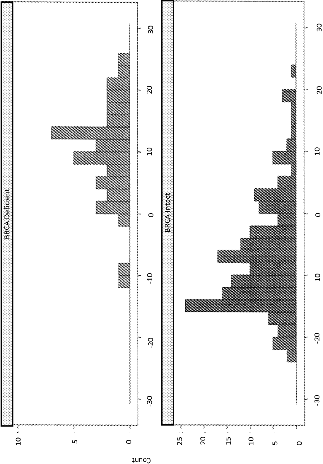
HRD-LST score
