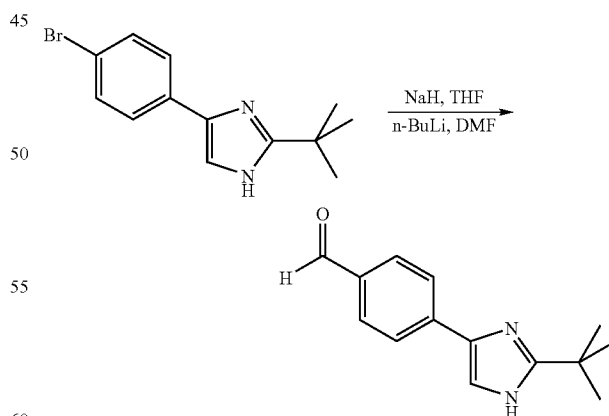
b) 4-[2-(1,1-dimethylethyl)-1H-imidazol-4-yl]benzaldehyde
