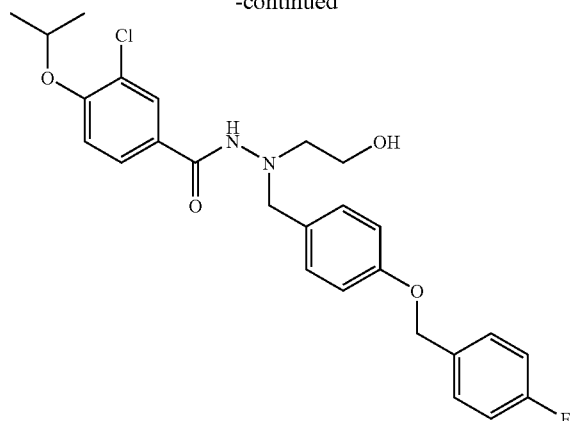
3-chloro-N'-[4-[[4-(1-methylethyl)oxy]phenyl]methyl]phenyl]methyl]-N'-(2-hydroxyethyl)-4-[(1-methylethyl)oxy]benzohydrazide
