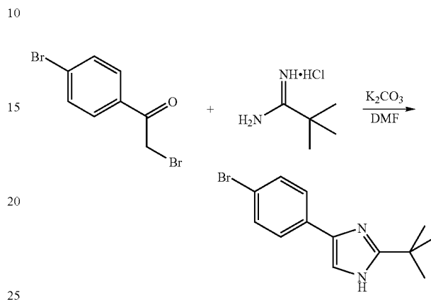
a) 4-(4-bromophenyl)-2-(1,1-dimethylethyl)-1H-imidazole
