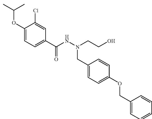
b) 3-chloro-N'-({4-[(1-methylethyl)oxy]phenyl}methyl)-N'-(2-hydroxyethyl)-4-[(1-methylethyl)oxy]benzaldehyde
