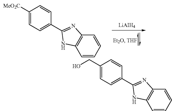
b) 4-(1H-benzimidazol-2-yl)phenylmethanol
