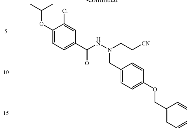
3-chloro-N'-(2-cyanoethyl)-4-[(1-methylethyl)oxy]-N'-({4-[(phenylmethyl)oxy]phenyl}methyl)benzohydrazide
