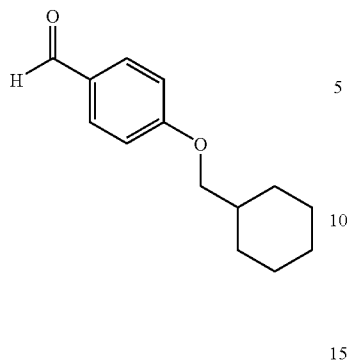
a) 4-[(cyclohexylmethyl)oxy]benzaldehyde
