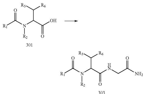
Reaction Scheme 3
