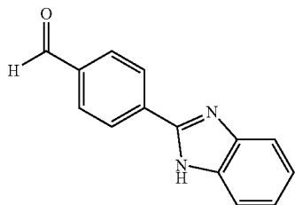
a) 4-(1H-benzimidazol-2-yl)benzaldehyde
