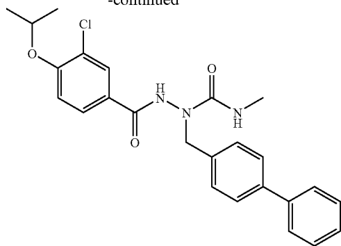
1-(4-biphenylmethyl)-2-({3-chloro-4-[(1-methylethyl)oxy]phenyl}carbonyl)-N-methylhydrazinecarboxamide
