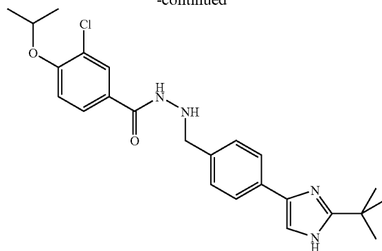
c) 3-chloro-N'-({4-[2-(1,1-dimethylethyl)-1H-imidazol-4-yl]phenyl}methyl)-4-[(1-methylethyl)oxy]benzohydrazide
