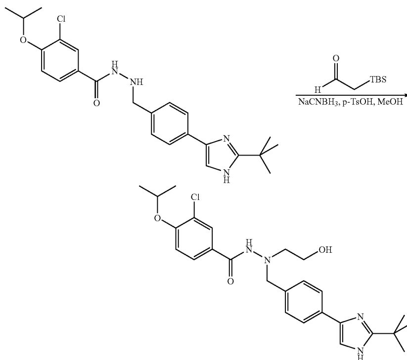
d) 3-chloro-N'-({4-[2-(1,1-dimethylethyl)-1H-imidazol-4-yl]phenyl}methyl)-N'-(2-hydroxyethyl)-4-[(1-methylethyl)oxy]benzohydrazide
