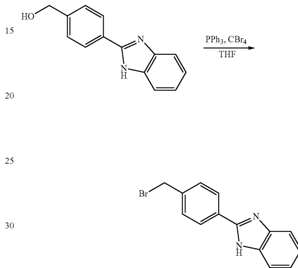
c) 2-[4-(bromomethyl)phenyl]-1H-benzimidazole
