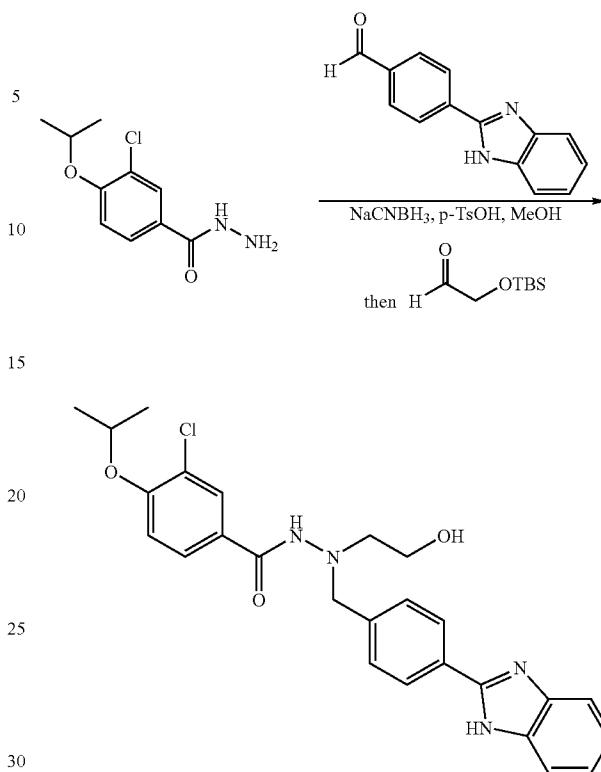
b) N'-{[4-(1H-benzimidazol-2-yl)phenyl]methyl}-3-chloro-N'-(2-hydroxyethyl)-4-[(1-methylethyl)oxy]benzohydrazide
