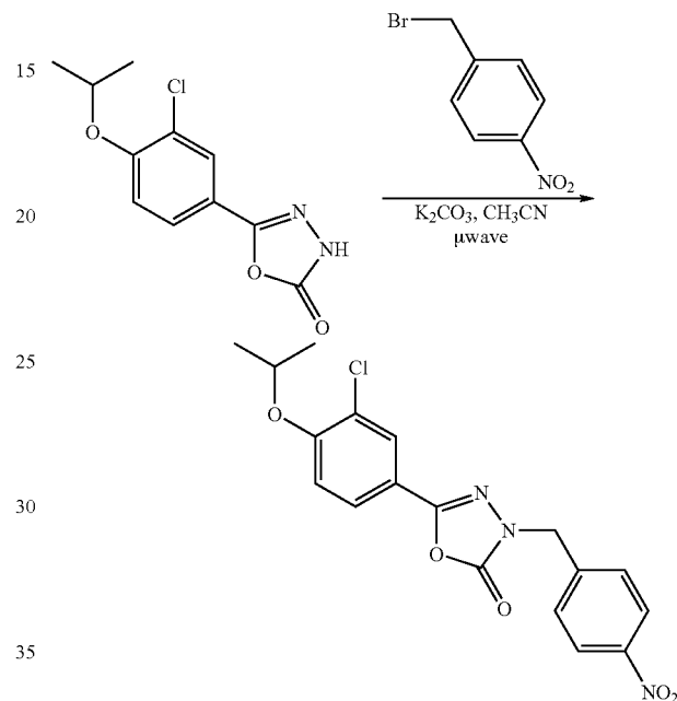
a) 5-{3-chloro-4-[(1-methylethyl)oxy]phenyl}-3-[(4-nitrophenyl)methyl]-1,3,4-oxadiazol-2(3H)-one
