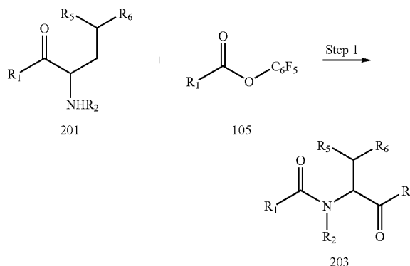
Reaction Scheme 2
