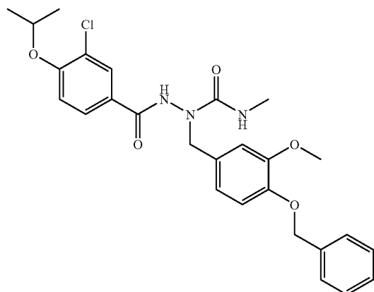
c) 2-({3-chloro-4-[(1-methylethyl)oxy]phenyl}carbonyl)-N-methyl-1-({3-(methyloxy)-4-[(phenylmethyl)oxy]phenyl}methyl)hydrazinecarboxamide
