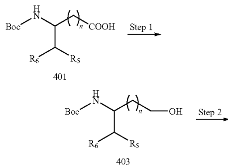
Reaction Scheme 4
