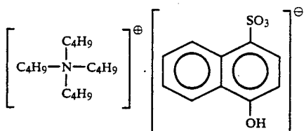
Exemplary Compound 1
