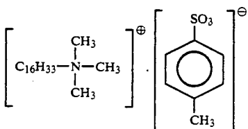
Exemplary Compound 2
