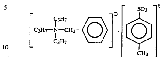
Exemplary Compound 6
