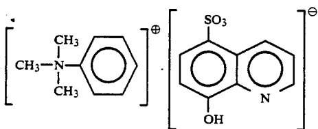
Exemplary Compound 5
