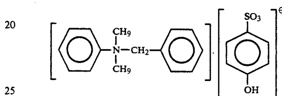
Exemplary Compound 7
