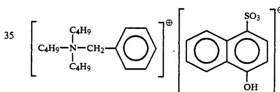
Exemplary Compound 8
