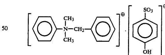
Exemplary Compound 9
