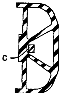
FIG. 18 (PRIOR ART)
