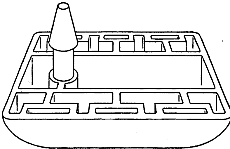
FIG. 55 (PRIOR ART)
