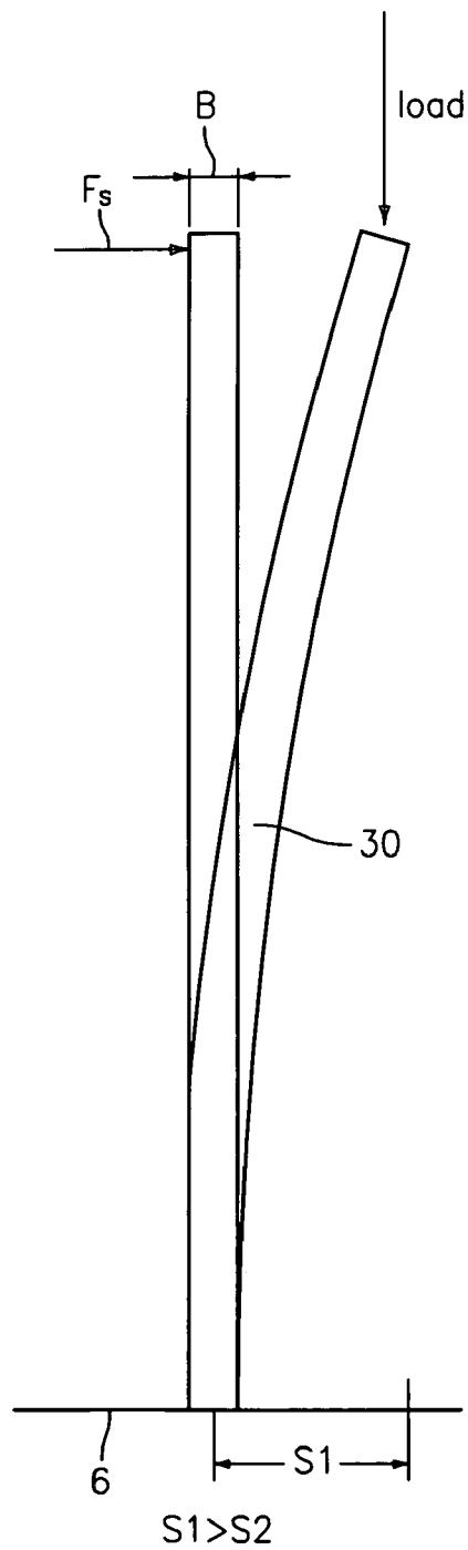
Front view of crane boom
