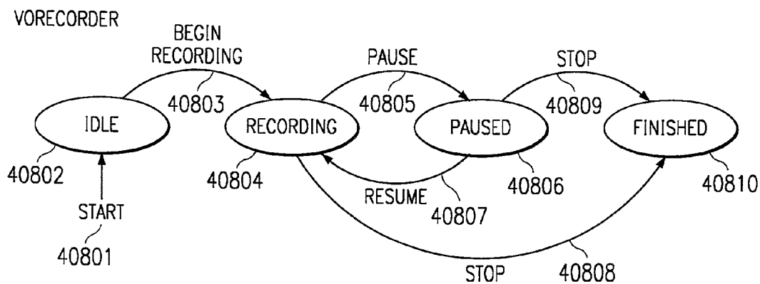
STATE TRANSITION DIAGRAM FOR VORECORDER'S STATE VARIABLE
