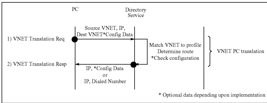
2. VNET PC queries a directory service for a VNET translation
