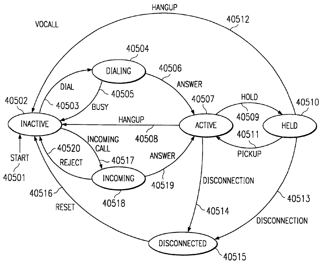
STATE TRANSITION DIAGRAM FOR VOCALL'S STATE VARIABLE
