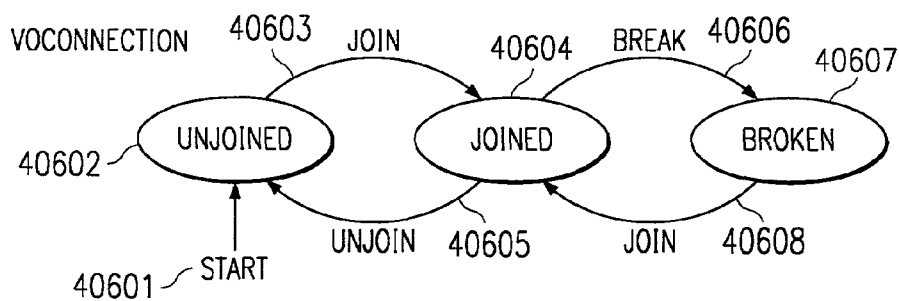
STATE TRANSITION DIAGRAM FOR VOCONNECTION'S STATE VARIABLE
