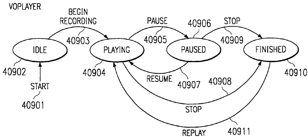
STATE TRANSITION DIAGRAM FOR VOPLAYER'S STATE VARIABLE
