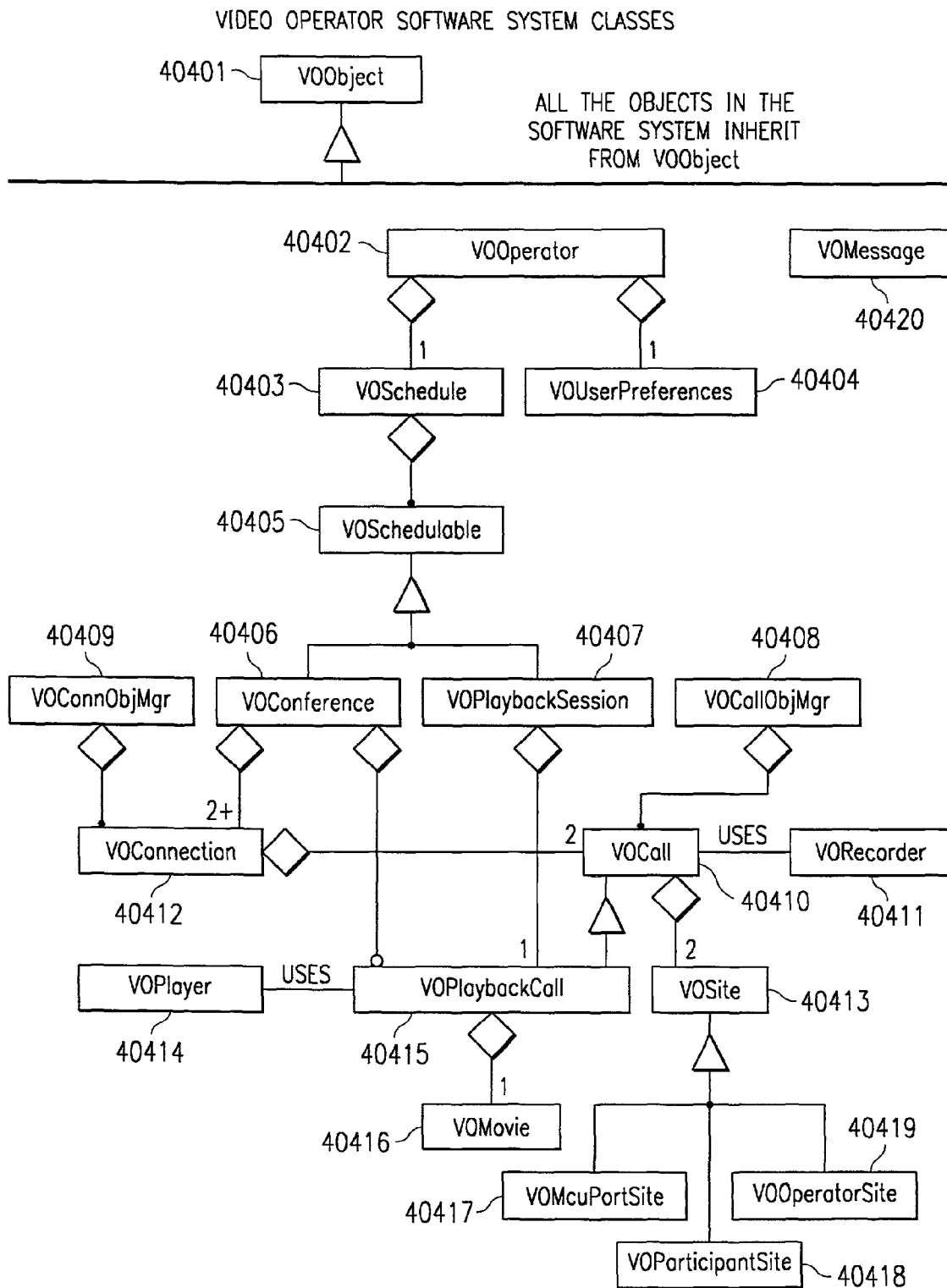
CLASS HIERARCHY FOR VIDEO OPERATOR SOFTWARE SYSTEM
