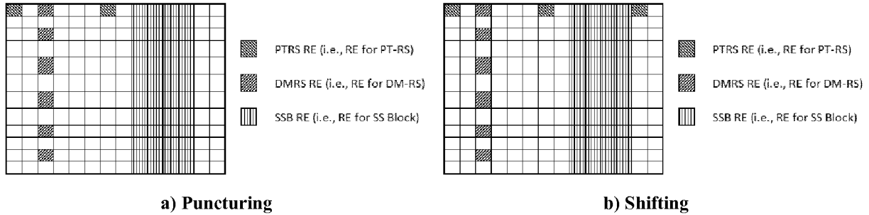
Figure 4. Examples of PTRS collision with SSB with PTRS time density 1/4.
