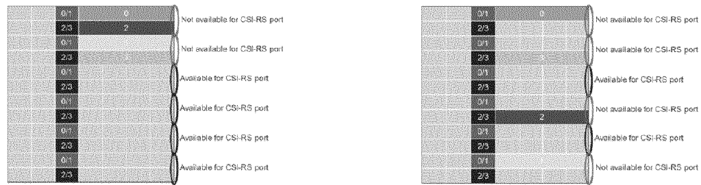
a) RE-level offset associated with DM-RS port index
