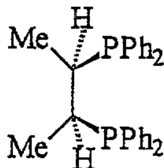
(S,S) - CHIRAPHOS
