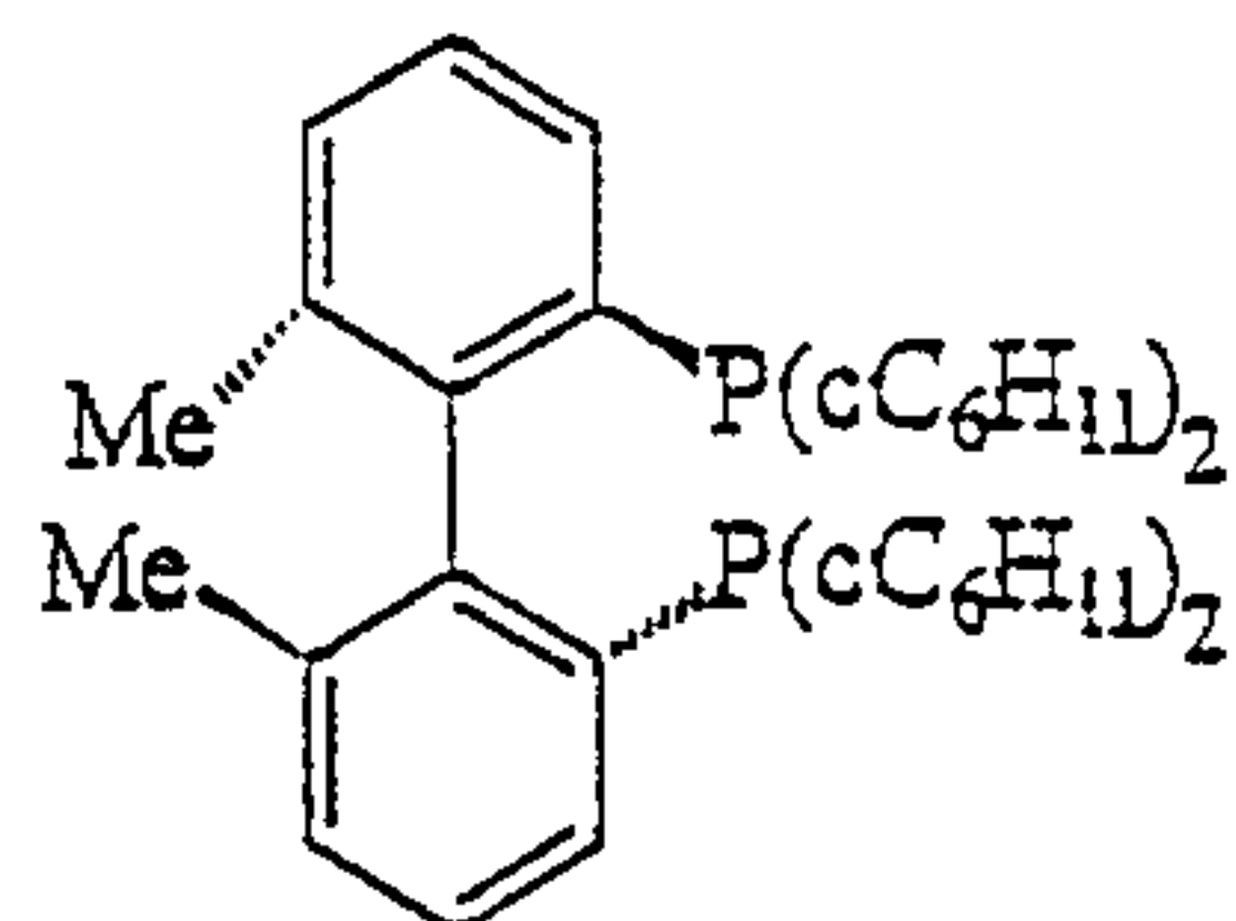
(R)-BICHEP
