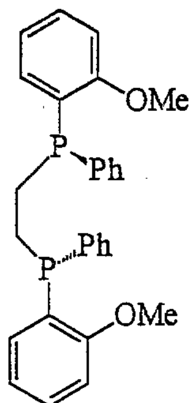
(R,R) - DIPAMP
