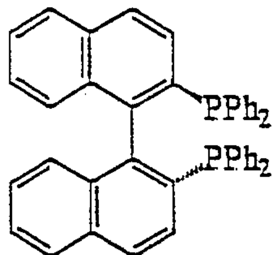
(R)-BINAP
