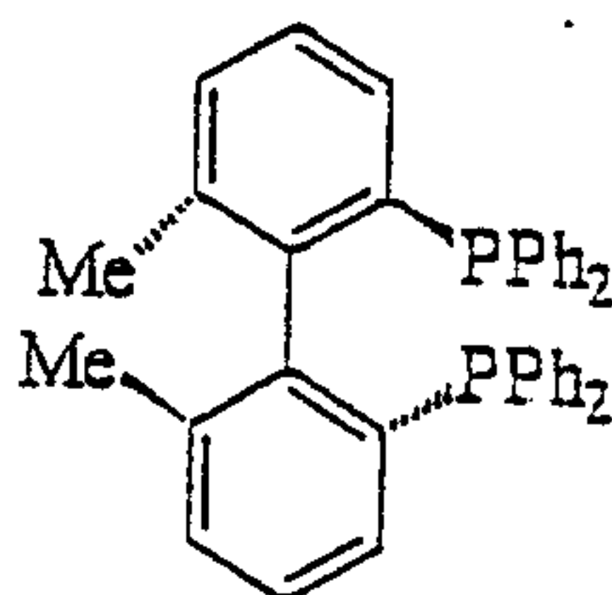
(R)-BICHEP
