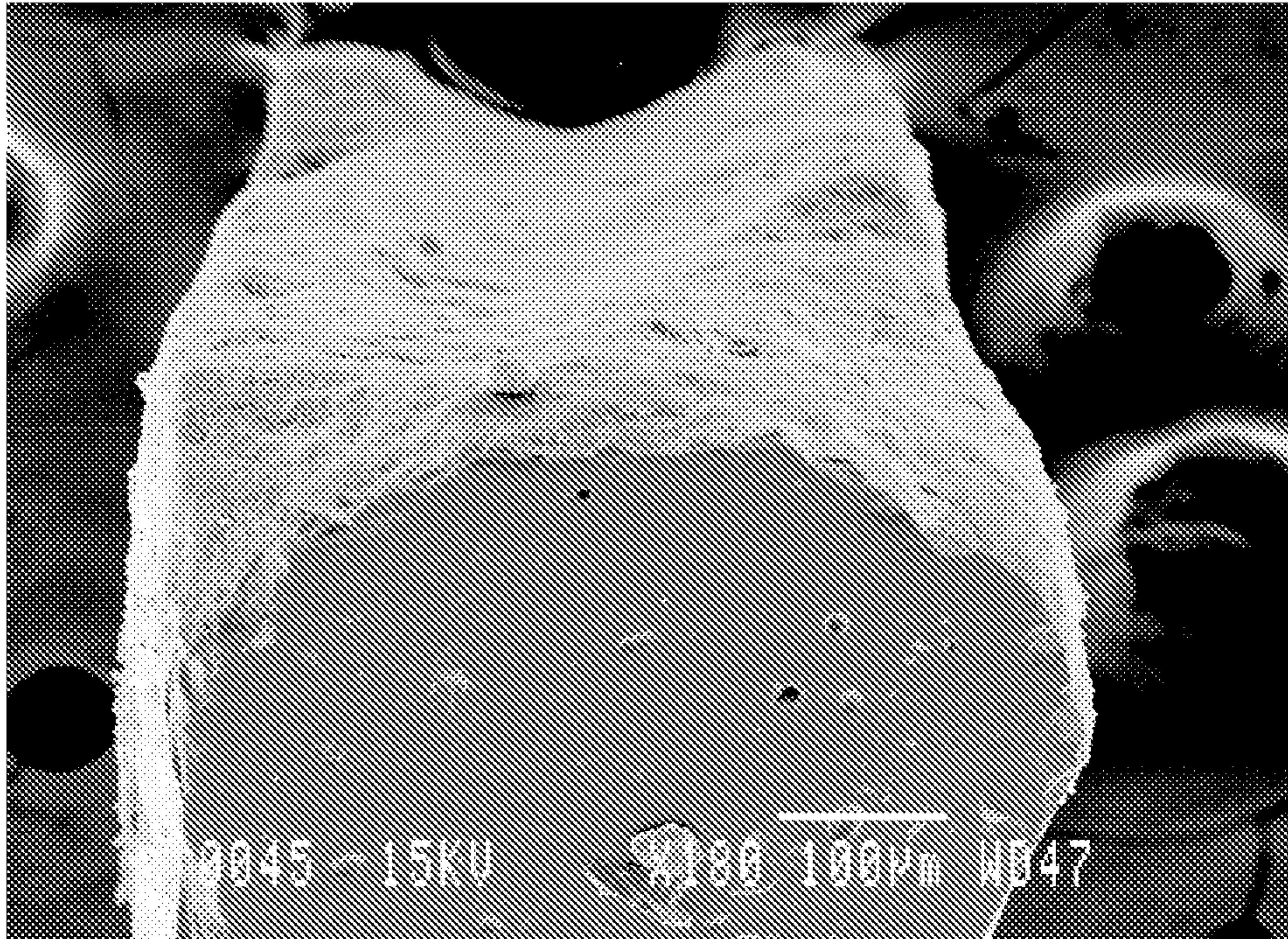
Fig. 10 PRIOR ART
