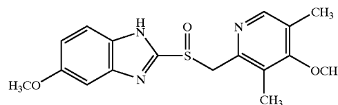
5-Methoxy
