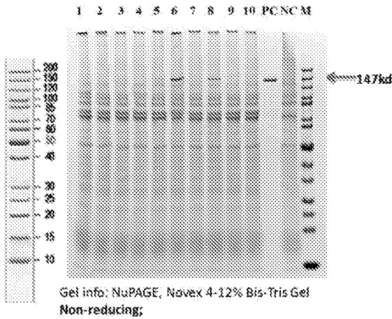
Non-reduced SDS-Page
