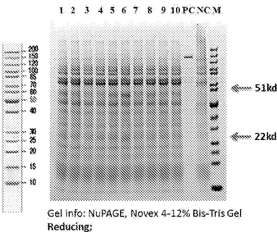
Reduced SDS-Page
