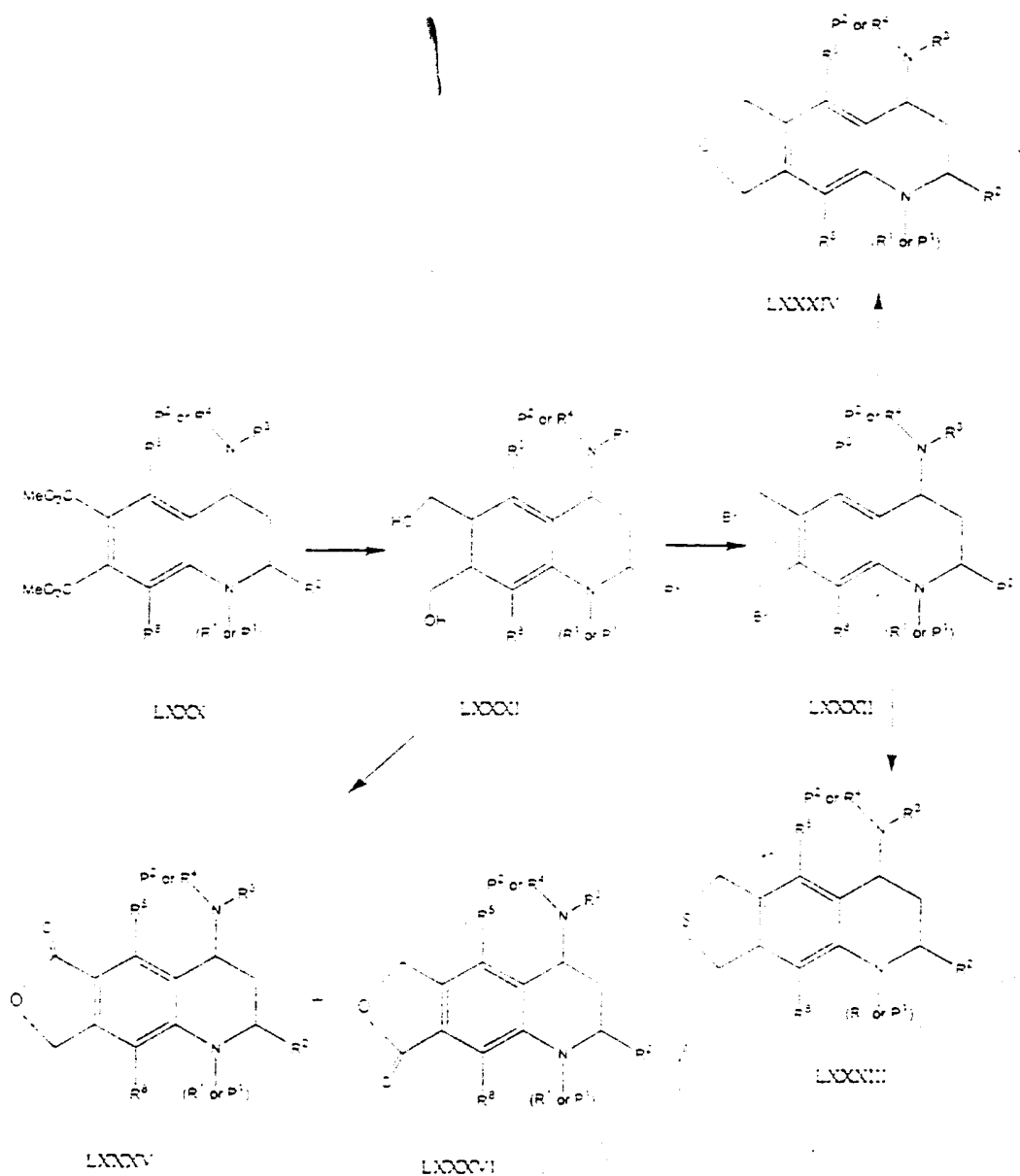
SCHEME VIII
