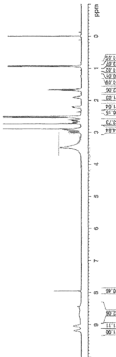
1 H NMR (500 MHz, DMSO-d 6 ) of Compound 10 (H 2 O)
