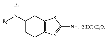
formula I_{(2HCl \cdot H_2O)}
